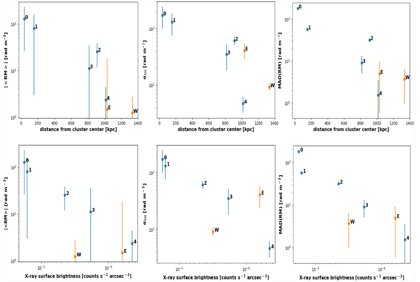
Figure 8. |\langle RM \rangle| , \sigma_{RM} , and MAD(RM) of the sources in the cluster computed in the B-configuration plotted against the projected distance of each source from the X-ray peak (top panels) and against the X-ray surface brightness at the position of each source (bottom panels). The uncertainties plotted for |\langle RM \rangle| and \sigma_{RM} are the \pm 1\sigma computed considering n_{beam} independent samples for each source. The uncertainties plotted for MAD(RM) are derived from the median error on the single RM measurement, med(\sigma_\phi) . The five sources detected in polarization are numbered as in Fig. 1 and the eastern and western relics are marked with the letters ‘E’ and ‘W’, respectively.
