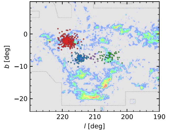
Figure 3. The CO emission map obtained from Dame et al. (2001) in the region where member candidates reside. The red dots are candidate members of LP 2439, and the blue dots are candidate members of NGC 2232. The purple and green dots represent the purple and green groups, respectively.
