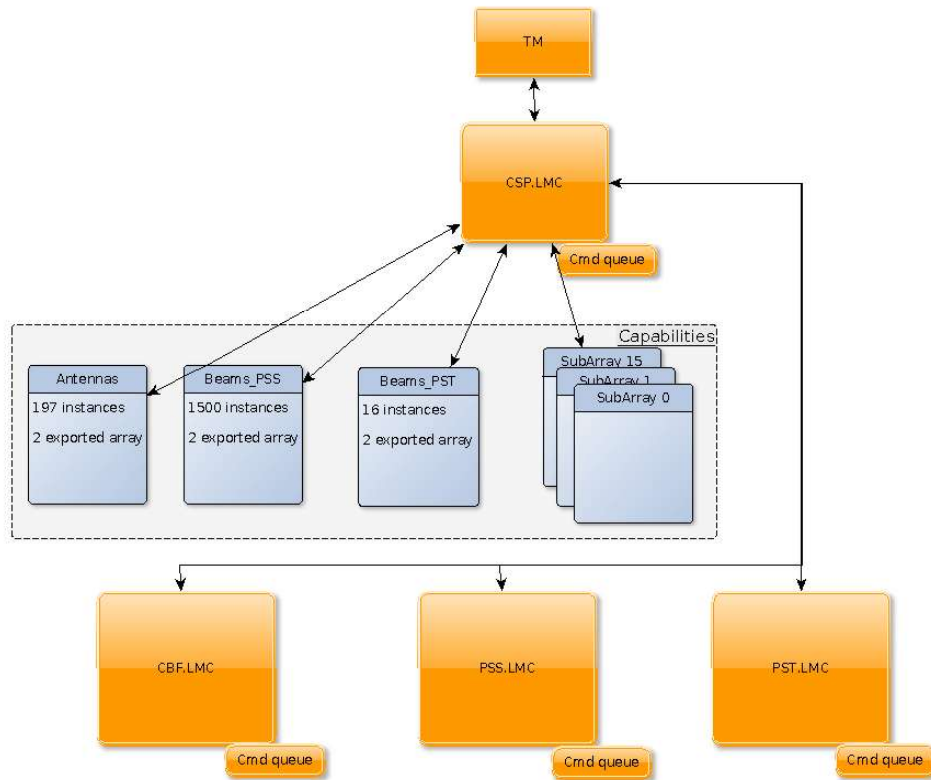
Figure 1. Basic Control Schema of a SKA element (CSP)
