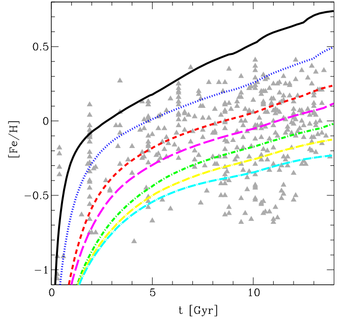
Figure 4. Temporal evolution of [Fe/H] for our best model REF1 with radial gas flows and variable SFE at different Galactocentric distances (curves; see Figure 3, upper panel, for the legend). Also shown are data by Bensby et al. (2014) for solar neighborhood stars (symbols).
