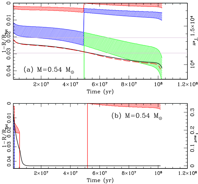
Figure 2. Time evolution of the HB convective regions for a track with Z = 0.006 , Y = 0.28 and M = 0.54\,M_{\odot} . Panel a (top) shows the standard evolution, panel b (bottom) shows the evolution including He-diffusion. The dashed regions represent the location of convection zones, in terms of fractional radius (values going from 0 in the atmosphere to 1 in the centre). The colours are red, blue and green in order, starting from the most external convective zone. The colours may change along the evolution if one or more specific convective regions appear or vanish when T_{\text{eff}} evolves. The T_{\text{eff}} as a function of time (scale to the right of panel a) is shown for the standard track (black full line) and the track including diffusion (red dashed). Two horizontal lines signal the standard G-jump ( 11\,500 K) and the anomalous G-jump T_{\text{eff}} = 13\,500 K. In panel b, the black line shows the evolution of Y_{\text{surf}} (scale on the right) in the track with diffusion. The track evolves from high to low T_{\text{eff}} , so the standard track has initially on top the He I partial ionization region, and below the He II region. At T_{\text{eff}} < 11\,500 K the partial H-ionization convection zone appears. In panel b, we see that the two He-convection regions disappear very soon, as helium settles in the layers where it would be partially ionized. Surface turbulence reappears suddenly below the standard G-jump, where hydrogen is no longer fully ionized. The atmospheres along this whole T_{\text{eff}} range have very small or negligible helium.
