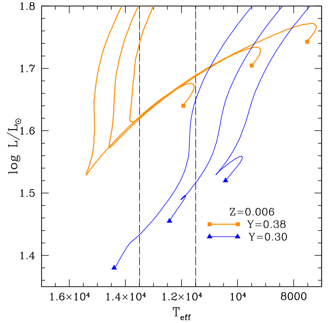
Figure 1. Comparison of the morphology of two different sets of stellar evolution tracks in the theoretical HR diagram. The ZAHB points are identified by squares for Y = 0.38 and triangles for Y = 0.30 . The standard and hotter G-jumps are marked by dotted black lines. From hotter to cooler ZAHB location, the masses of the tracks are 0.53 , 0.54 and 0.55 M_{\odot} for both Y values. These tracks do not include helium settling, to display the prime effect of the initial helium content in the evolution.
