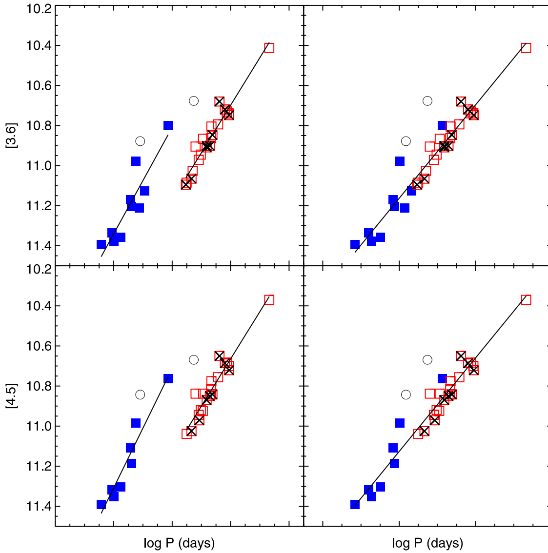
Figure 7. IRAC period–luminosity relations for M4 RR Lyrae stars. (Left) FO (blue filled squares) and FU (red open squares) variables are fit independently (black solid lines). (Right) single fit with fundamentalized FO RR Lyrae stars. All magnitudes are corrected for extinction. Random uncertainties in the average magnitudes of all variables are smaller than the symbols used and are not shown. Candidate Blazhko stars are marked with black crosses. The open circles mark the positions of the two stars (V20 and V21) that were not included in the fit of the PL relation due to blends with nearby sources.
