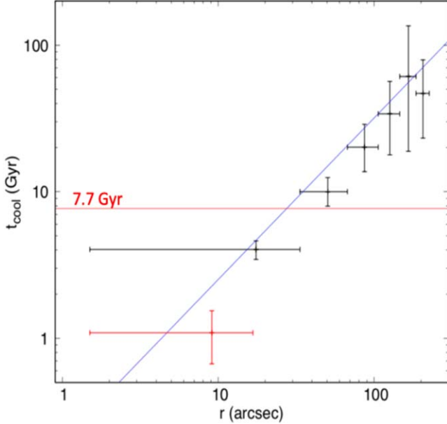
Figure 8. Cooling time profile for A2495. Each point represents the cooling time value for one of the annular regions used for the spectral extraction, and the x-axis error bars are the lower and upper limits of each ring. The red line represents t_{\text{age}} = 7.7 Gyr, while the blue line is the best fit of the profile: t_{\text{cool}} = 0.199r^{1.102} . The red point is derived from the spectral analysis described in Section 4.3.
