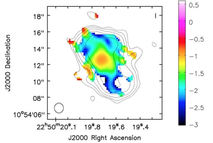
Figure 3. Spectral index map of A2495 between 5 and 1.4 GHz. Contours are the same as in the 1.4 GHz map, and typical errors range from \Delta\alpha \simeq 0.2 to \Delta\alpha \simeq 0.6 for the inner and outer regions, respectively.
