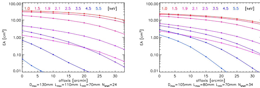
Fig. 7. Effective area (EA) as a function of off-axis location for the large (left) and small (right) designs. The different colored curves are for different photon energies, as in Figure 5. A different projection of the same information, EA vs. energy for different off-axis angles is shown in Figure 8.
