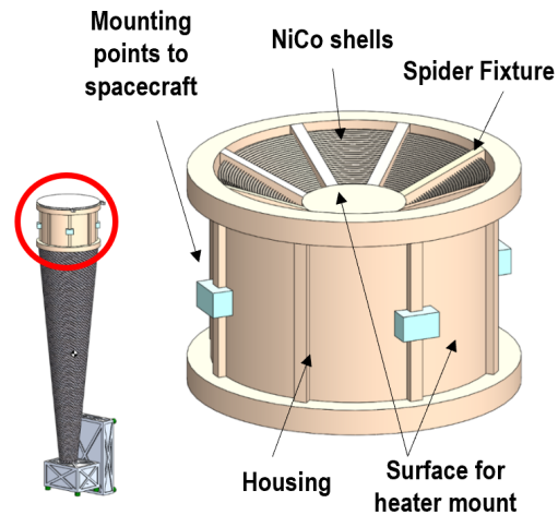
Fig. 2. Mirror module design of the MiXO for the CubeX XIS. The two configurations of nested shells we adopt are discussed in Section 3.
