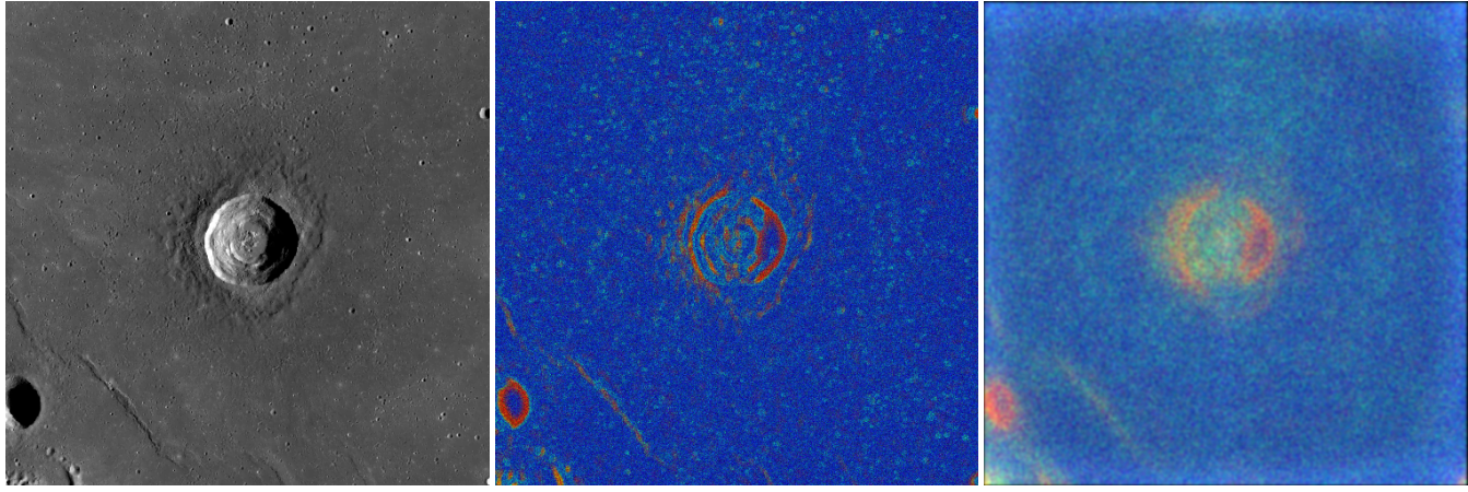
Fig. 10. Demonstrating the performance of CubeX with a raytrace of a 100 km wide region around Picard crater at North-East of the Moon. (Left:) An optical image taken with Lunar Reconnaissance Orbiter (LRO). (Middle:) Mock-up of a nominal emission map of X-ray XRFs (see text). (Right:) A raytrace of a 500 ksec observation of the region with CubeX . The X-ray raytrace image is made with Fe-L (red), Mg-K (green), and Al-K (blue) lines. The composition of the region is assumed to be a varying composite of lunar mare basalt (higher Fe and Mg abundances) and anorthositic breccia meteorite (higher Al abundance). The composition variation at 1 - 3 km scales is easily detectable with the MiXO.
