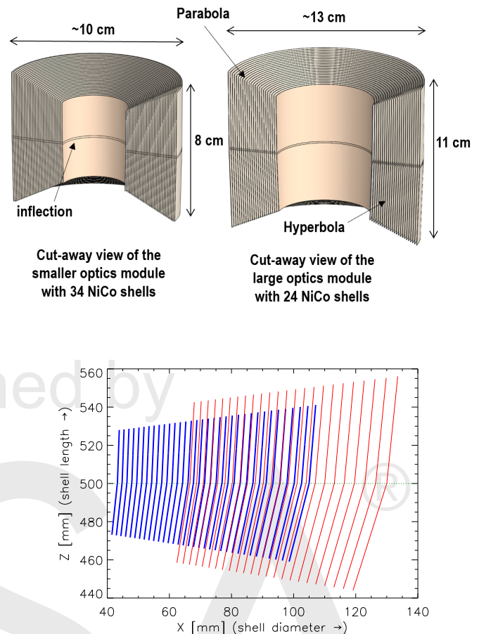
Fig. 4. Sketches of the CubeX tapered configurations drawn to scale. The cut-away views of the small (top left) and large (top right) configurations are also shown. The lower panel shows a line drawing cut-out of the profiles, with the large (red) and compact (blue) shells superposed. The horizontal dotted line indicates the focal length.
