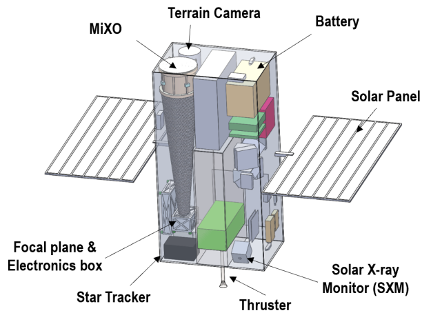
Fig. 1. CubeX spacecraft: CubeX is designed to be a secondary payload, weighing about 43 kg in a 35 × 23 × 68 cm volume. The X-ray Imaging Spectrometer (XIS) is at the front/left of the figure, spanning almost the full length of the configuration. The focal length of the baseline design of the XIS is 70 cm. See also Figure 2 for a close-up of the X-ray mirror assembly of the Miniature X-ray Optics (MiXO) in the XIS.
