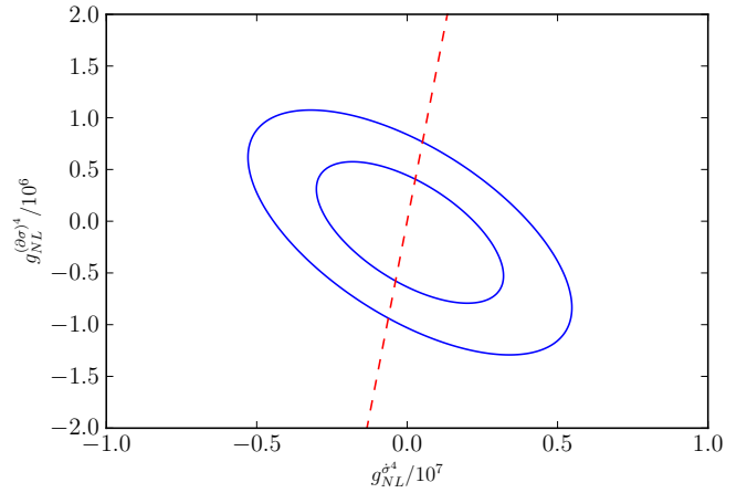
Fig. 33. 68% and 95% confidence regions in the (g_{\text{NL}}^{(4)}, g_{\text{NL}}^{(4\partial\partial)}) plane, with the Lorentz invariant model in Eq. (107) shown as the dashed line.
