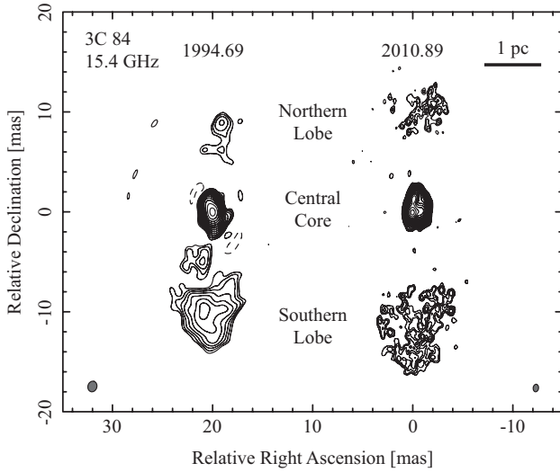
Fig. 3 VLBA images of 3C 84 obtained at 15.4 GHz. Images refer to observations performed on 1994 September 10 (left) and 2010 November 20 (right). The lowest contour is three times the off-source rms noise (one \sigma ), and the contour levels are -3\sigma , 3\sigma \times (\sqrt{2})^n ( n = 0, 1, 2, \dots ). The peak intensity is 5.86 \text{ Jy beam}^{-1} (left) and 5.54 \text{ Jy beam}^{-1} (right). The restoring beam is indicated in the bottom left/right corner of the left/right images. The total flux density of northern and southern lobes are 0.8 Jy and 6.7 Jy in 1994, while they decrease to 0.5 Jy and 1.4 Jy in 2010, respectively.
