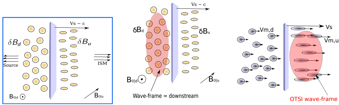
Figure 8. Left panel: Magnetic field structures around the shock front. The shock propagates from the left to the right. In the upstream region magnetic disturbances are anisotropic with coherence length along the shock normal being much larger than in the transverse one (along the plane of the shock front). Downstream, the turbulence is compressed at the shock front and magnetic disturbances should be roughly isotropic with a single coherence length in all directions. Middle panel: wave-frame of magnetic turbulence downstream. Right panel: wave-frame of upstream turbulence, with non-zero velocity relative to the shock (illustrated in the particular case of the oblique two-stream instability (OTSI), see text). Also, v_{d,m} ( v_{u,m} ) is the velocity of downstream (upstream) electromagnetic irregularities relative to the upstream (lab) frame.
