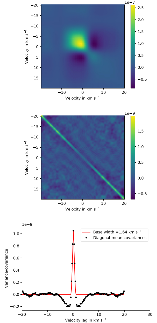
Figure B1. Upper panel: reduced-rank ( k_{\text{max}} = 10 ) covariance matrix of the sequence of CCFs residuals, showing the large-scale covariance due to profile variability. Middle panel: Residual covariance matrix obtained by subtracting the reduced-rank representation from the full covariance matrix. Lower panel: Mean residual covariance along diagonals as a function of horizontal velocity offset from the leading diagonal. The diagonal ridge is triangular in cross-section, with base width 1.64 \text{ km s}^{-1} , which is equivalent to two physical pixels on the spectrograph CCD.
