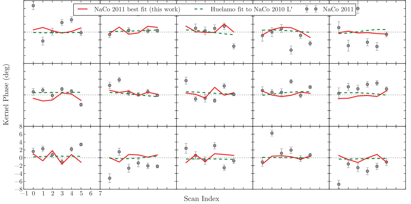
Figure 21. Kernel phase data for 2011 NaCo Ks observations, shown with best fits from this work (red line) and Huelamo et al. (dashed green line). Each subplot corresponds to a single linear combination of closure phases plotted against scan index (a proxy for sky rotation angle). The error bars plotted are unscaled, while our parameter constraints are derived using error bars scaled such that the reduced \chi^2 of the best fit model is equal to 1.
