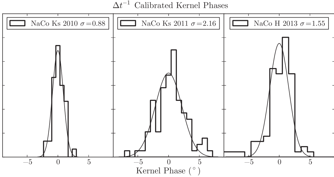
Figure 11. Normalized histograms of calibrated NaCo 2010 and 2011 Ks as well as NaCo 2013 H kernel phases, with their best fit Gaussian distributions over plotted. These calibrated kernel phases have much higher scatter than the other data sets. The Gaussian distributions were used to generate noise realizations for the simulations described in Section 7.
