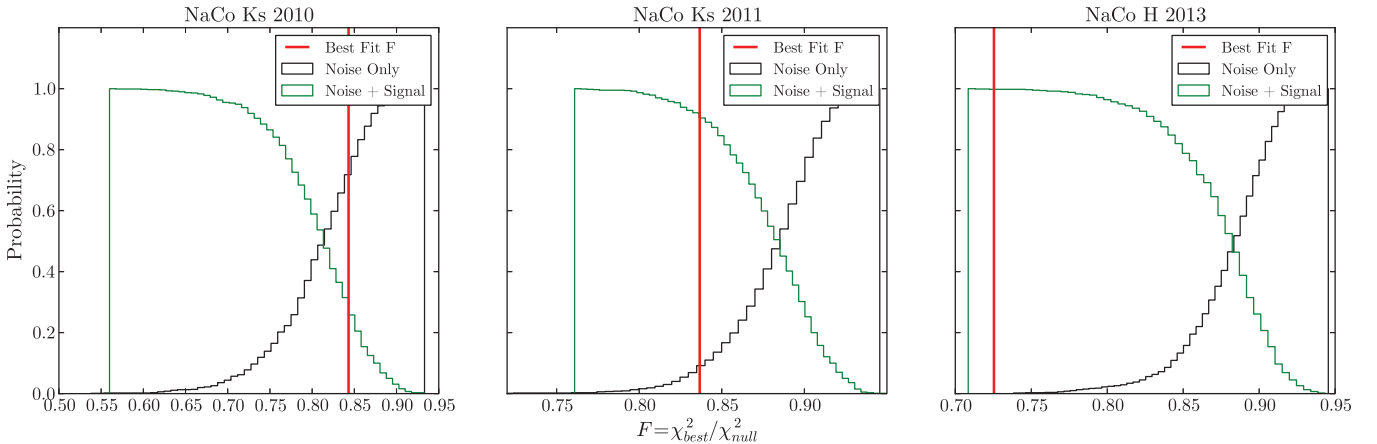
Figure 13. False alarm testing for 2010 and 2011 Ks and 2013 H band observations. In each panel, the black cumulative histogram shows the F statistics (best fit \chi^2 divided by null model \chi^2 ) for 1000 noise simulations. The intersection of the red vertical line with the black histogram yields a false alarm probability. The green cumulative histogram shows the F statistics from the 1000 noise + signal simulations carried out for each set of observations. The intersection of the red line with this histogram gives the fraction of noise + signal simulations that look less significant (higher F statistic) than the best fit.
