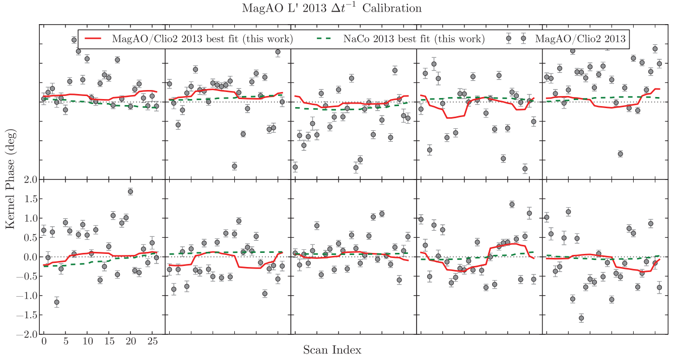
Figure 19. Kernel phase data for 2013 MagAO L' observations, shown with best fits from this work (red line) and the NaCo 2013 L' best fit (dashed green line). Each subplot corresponds to a single linear combination of closure phases plotted against scan index (a proxy for sky rotation angle). The error bars plotted are unscaled, while our parameter constraints are derived using error bars scaled such that the reduced \chi^2 of the best fit model is equal to 1.
