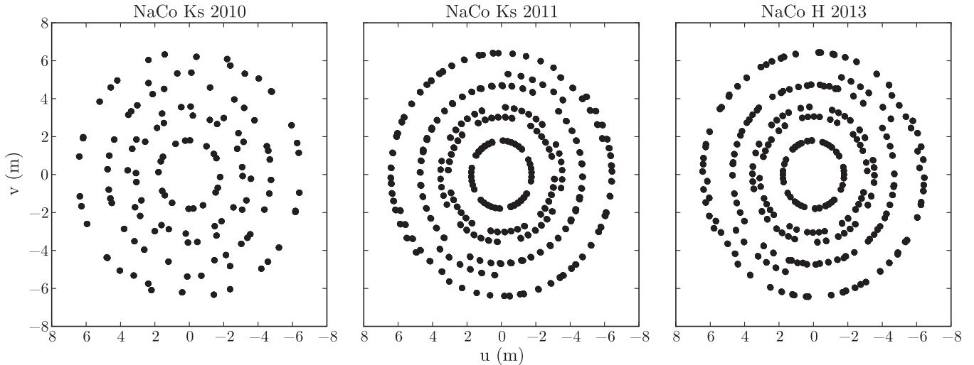
Figure 9. Sky rotation comparison in (u, v) space for 2010 and 2011 NaCo Ks data as well as 2013 NaCo H data. The NaCo 2010 and 2011 Ks data had changes in sky rotation of \sim 19^\circ and \sim 38^\circ , respectively. The sky rotation in the NaCo 2013 H data was \sim 39^\circ .
