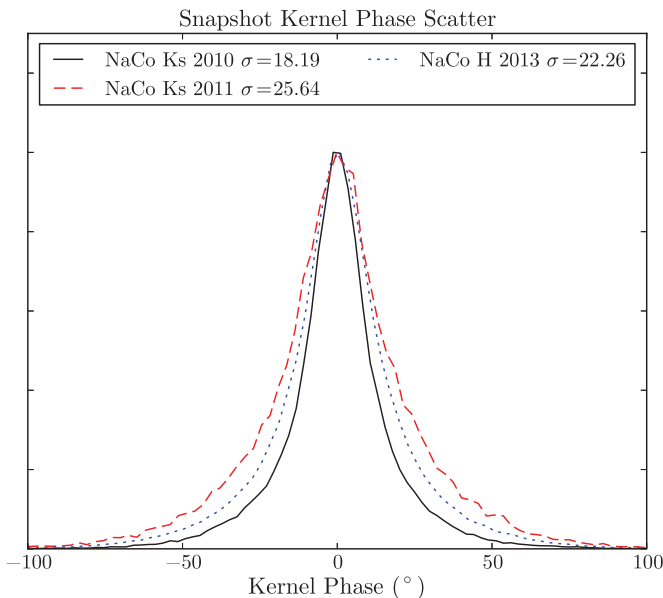
Figure 10. Normalized histogram of uncalibrated kernel phases for 2010 and 2011 Ks as well as 2013 H band data. For a subset of each dither (taken so that equal amounts of integration came from each observation), we subtract the mean kernel phase from each individual measurement to generate the histogram shown above. The snapshot errors for these data sets are significantly larger than those for the other six.
