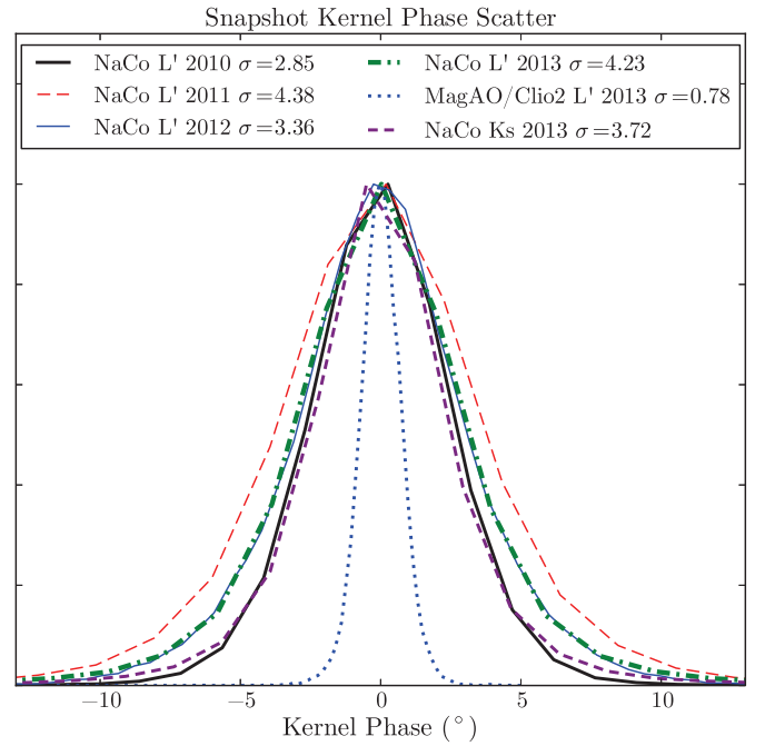
Figure 2. Normalized histograms of uncalibrated kernel phases for L' and 2013 Ks data. For a subset of each dither (chosen so that equal amounts of integration came from all observations), we subtract the mean kernel phase from each individual measurement to generate the histograms shown above. The snapshot kernel phase errors are much lower in the MagAO/Clio2 data than in the NaCo data sets, indicating lower levels of random noise.
