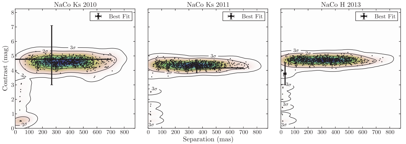
Figure 12. Noise simulations for all H and Ks data sets. The scattered points show the best fits to 1000 noise realizations for each data set, drawn from the Gaussian distributions shown in Figure 11. The color shows the probability distribution interpolated from the best fits, while the contours indicate 1\sigma , 2\sigma , and 3\sigma confidence intervals. The bold point with error bars represents the best fit for each epoch.
