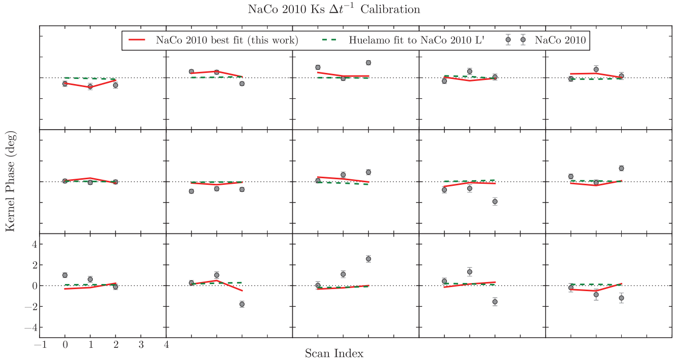
Figure 20. Kernel phase data for 2010 NaCo Ks observations, shown with best fits from this work (red line) and Huelamo et al. (dashed green line). Each subplot corresponds to a single linear combination of closure phases plotted against scan index (a proxy for sky rotation angle). The error bars plotted are unscaled, while our parameter constraints are derived using error bars scaled such that the reduced \chi^2 of the best fit model is equal to 1.
