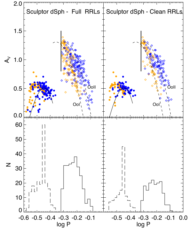
Figure 6. Top. Period-amplitude or Bailey diagrams for the full (left-hand panels) and for the clean (right-hand panels) samples of RRL stars in Sculptor. Open diamonds and filled circles represent RRAb and RRC, respectively. The dashed lines are the relations for RRAb stars in Oo-I and Oo-II clusters obtained by Cacciari, Corwin & Carney (2005) for the M3 RRAb variables. The solid curve is derived from the M22 (Oo-II cluster) RRC variable study by Kunder et al. (2013). Black vertical lines mark the HASP limit defined by Fiorentino et al. (2015a). Bottom. Period histograms for those RRL stars shown in the top panels. RRAb and RRC are shown as histograms with solid and dashed lines, respectively. For the sake of clarity, RRd stars are not plotted as their periods are less certain.
