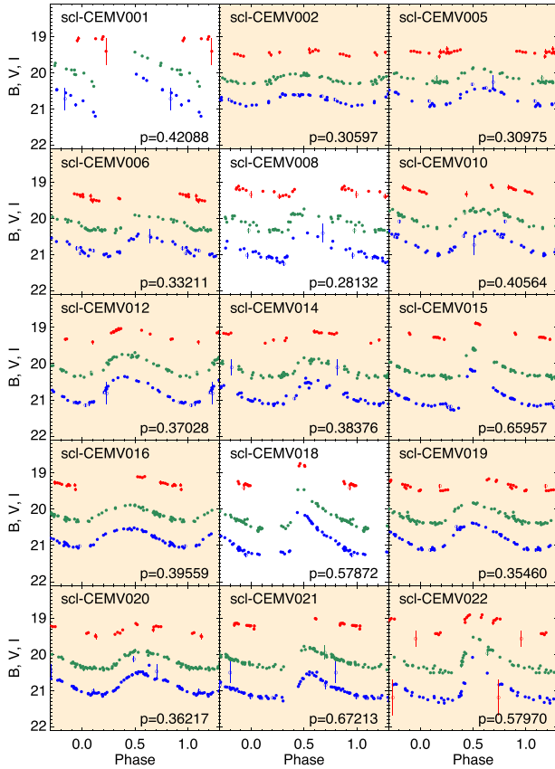
Figure 4. Sample of LCs of the RRL stars in the B (blue), V (green) and I (red) bands, phased with the period in days given in the lower-right corner of each panel. The name of the variable is given in the left-hand corner of each panel. Open symbols show the bad data points, i.e. with errors larger than 3\sigma above the mean error of a given star; these were not used in the calculation of the period and mean magnitudes. For clarity, the B and I LCs have been shifted by 0.4 mag down- and upward, respectively. Tinted backgrounds mark those RRL stars classified as members of the clean sample. All LCs are available as Supporting Information with the online version of the paper.
