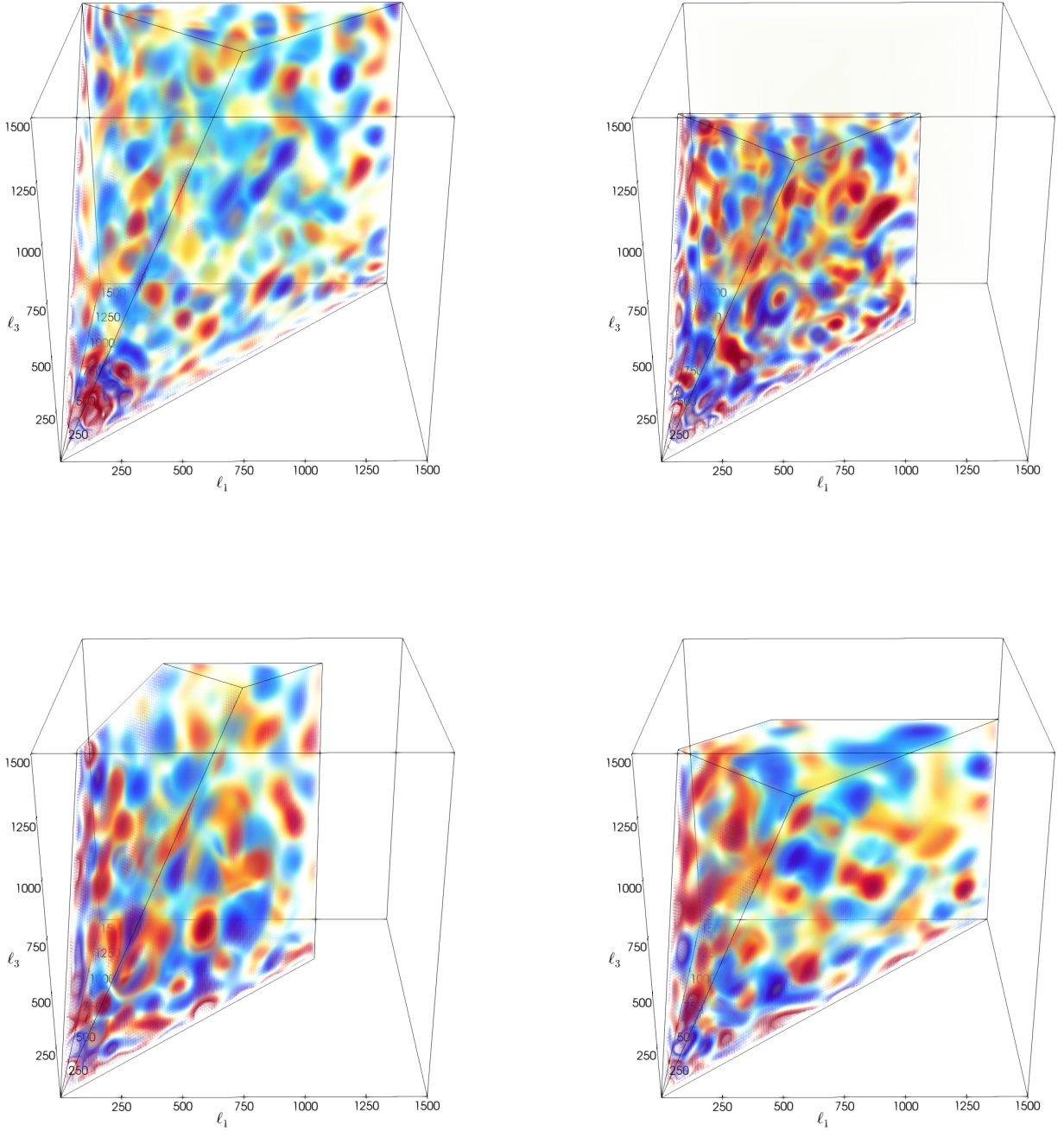
Fig. 10. Signal-to-noise-weighted temperature and polarization bispectra obtained from Planck SMICA maps using the Modal reconstruction with n_{\text{max}} = 2001 polynomial modes. The bispectra are (clockwise from top left) the temperature TTT for \ell \leq 1500 , the E -mode polarization EEE for \ell \leq 1100 , the mixed temperature/polarization TEE (with T multipoles in the z -direction), and lastly TTE (with E multipoles in the z -direction). The S/N thresholds are the same between all plots.
