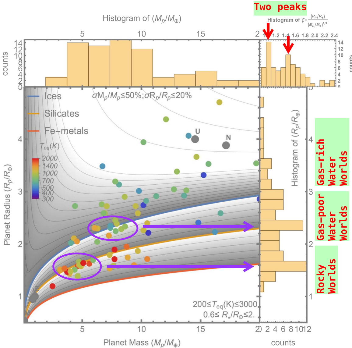
Figure 14. Mass–radius plot of all ( 200\text{ K} \leq T_{\text{eq}} \leq 3000\text{ K} ) small exoplanets with fractional radius errors less than 20% and fractional mass errors less than 50%. The bimodality in exoplanet radius distribution, as well as the \zeta -parameter, is distinct. The truncation of exoplanet mass distribution at \sim 11 M_{\oplus} is another prominent feature. We circle the likely m – r parameter domain, which gives rise to the two peaks. Not surprisingly, they are exactly what we had expected from our previous work (Zeng et al. 2019). The two tight clusters of exoplanets show a shift of about double the planet masses and (almost) double the planet radii: (1) a typical super-Earth is 3 – 5 M_{\oplus} , slightly bigger than Earth, and (2) a typical water world is 6 – 10 M_{\oplus} , slightly larger than 2.0 R_{\oplus} .
