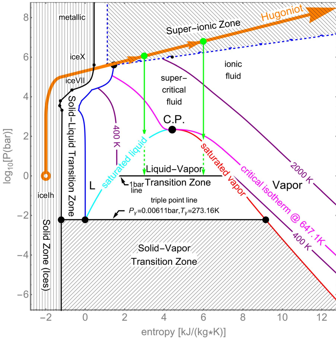
Figure 13. Entropy–pressure graph of water. It shows the \text{H}_2\text{O} phase diagram in the entropy vs. pressure space. The X-axis is the linear scale of entropy in units of [\text{kJ}/(\text{kg}\cdot\text{K})] , normalized to zero at the Ice Ih–liquid–vapor triple point. The Y-axis is log base 10 of pressure in bar ( 10^5 Pa). The hatched regions include (1) solid-vapor transition zone at the bottom, (2) the solid zone (including all forms of crystal ices) to the left, and (3) the superionic zone where protons are mobile within an oxygen crystal lattice on the top. The unhatched region corresponds to the fluid, which includes both liquid and vapor, and the vapor dome, which is the coexistence region between liquid and vapor phases. Above the C.P., supercritical fluid exists, together with ionic fluid at higher temperatures. Three isotherms are shown: 400, 647.1 (at critical temperature), and 2000 K. An example of Hugoniot (shock compression curve) is shown together with two examples of subsequent pressure-release curves (green vertical downward-pointing arrows).
