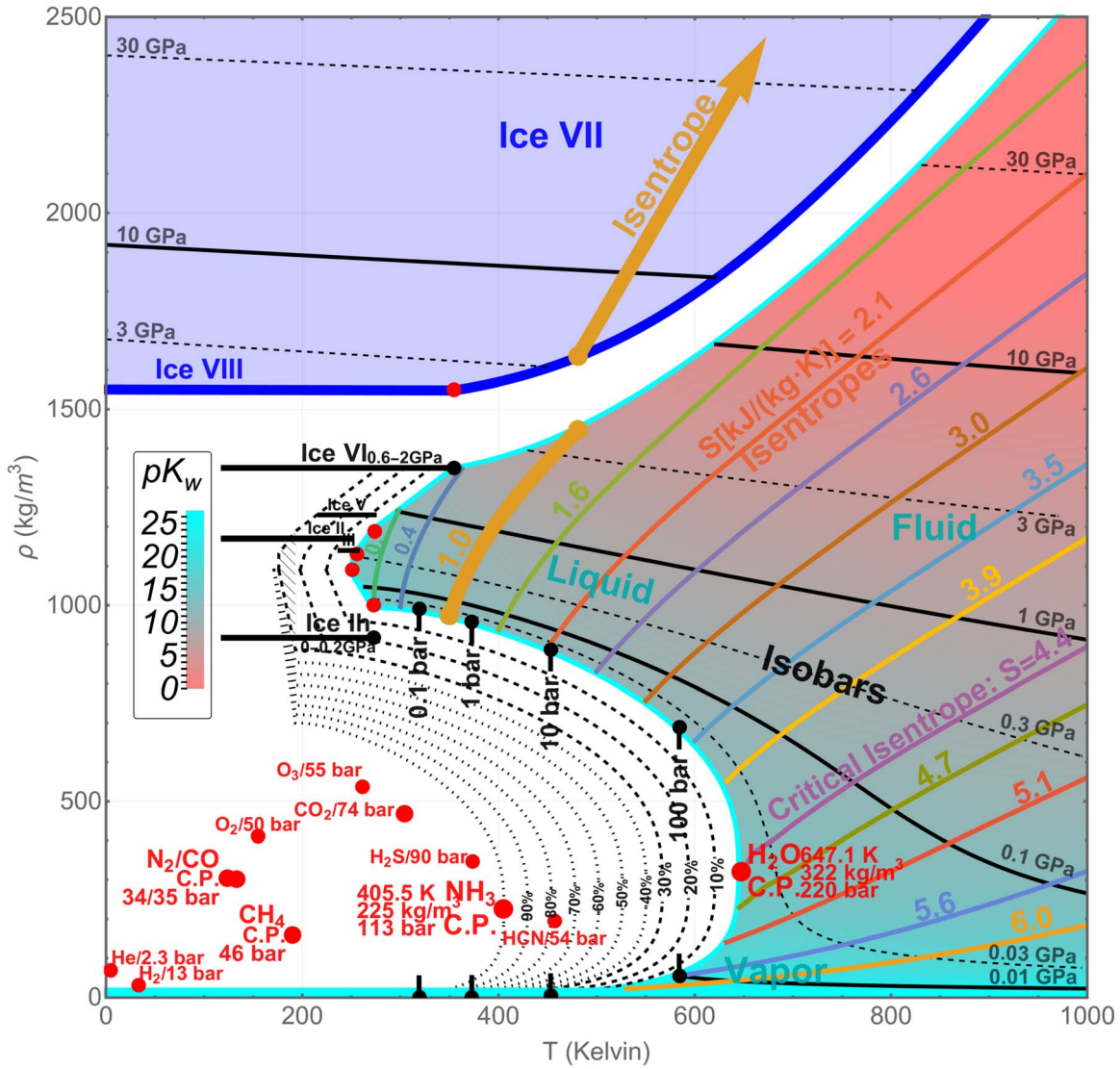
Figure 11. Temperature–density graph of water (zoomed in). It shows the H 2 O phase diagram in the temperature vs. density space. The X-axis is the linear scale of temperature in units of kelvin. The y-axis is the linear scale in density in units of kg m -3 . The colored zones include (1) the fluid zone on the right that includes liquid, vapor, and supercritical fluid, (2) the extensive solid zone on the top, and (3) ice-polymorphs (Ice I (hexagonal), Ice II, Ice III, Ice V, and Ice VI) with distinct densities on the left simplified and depicted as horizontal solid black lines. Within (1) and (2), isobars (contours of constant pressures) are shown in black as labeled, and isentropes (contours of constant specific entropy) are shown in color as labeled. The background coloring of the entire fluid zone is according to the calculated ionization constant ( pK_w ). The C.P. of H 2 O and the C.P. of some other selected simple substances are shown, in particular, ammonia NH 3 . The gradual change of C.P. with its associated boundary of the vapor–liquid coexistence curve (vapor dome, dashed as labeled) of the H 2 O–NH 3 mixture is also depicted.
