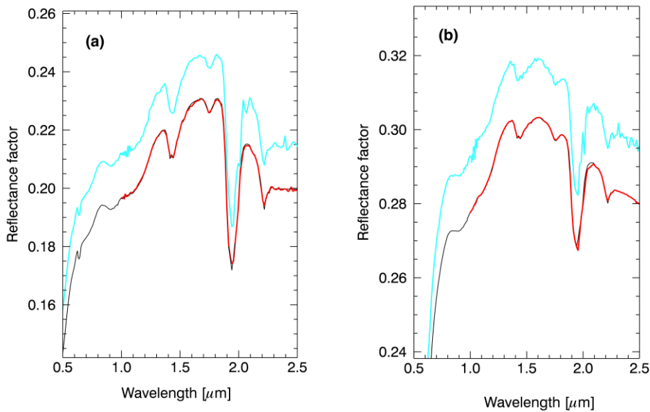
Figure 5. (a) Spectrum whose surface reflectance is made by 1% of bright component and 99% of dark component. (b) Spectrum whose surface reflectance is made by 50% of dark component and 50% of bright component. The retrieved surface reflectances are the red line over imposed to the true surface reflectance (black line). Shifted for clarity the
