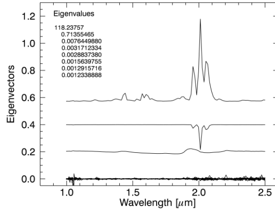
Figure 2. Eigenvectors retrieved using PCA for the simulated dataset, shifted for clarity. Only the first eight eigenvalues are listed.
