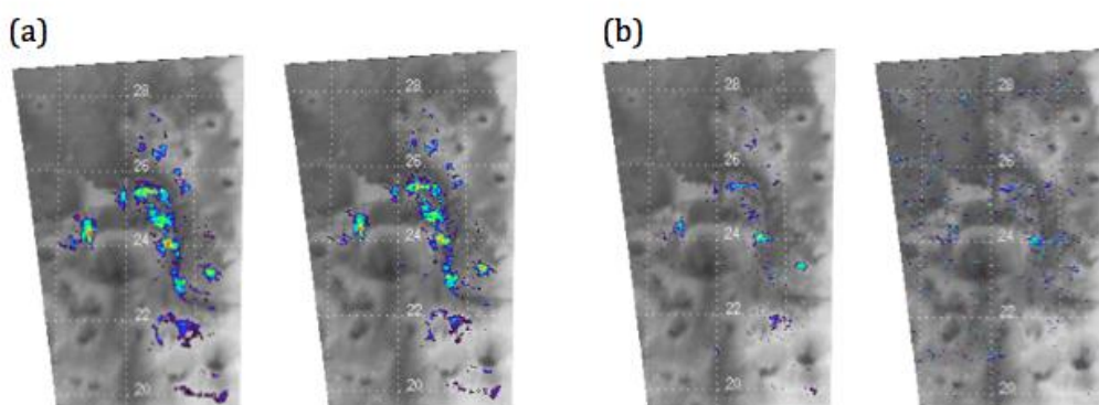
Figure 17: (a) Albedo map at 1 \mu\text{m} superimposed with the spectral index maps of the 1.93 \mu\text{m} band obtained considering surface reflectance with SAS method (on the left, using as threshold the 3\sigma of Gaussian distribution of values) and with MO method (on the right, considering a detection threshold of 2%). (b) Albedo map superimposed with spectral index maps of the 2.3 \mu\text{m} band obtained considering surface reflectances with SAS method (on the left,
