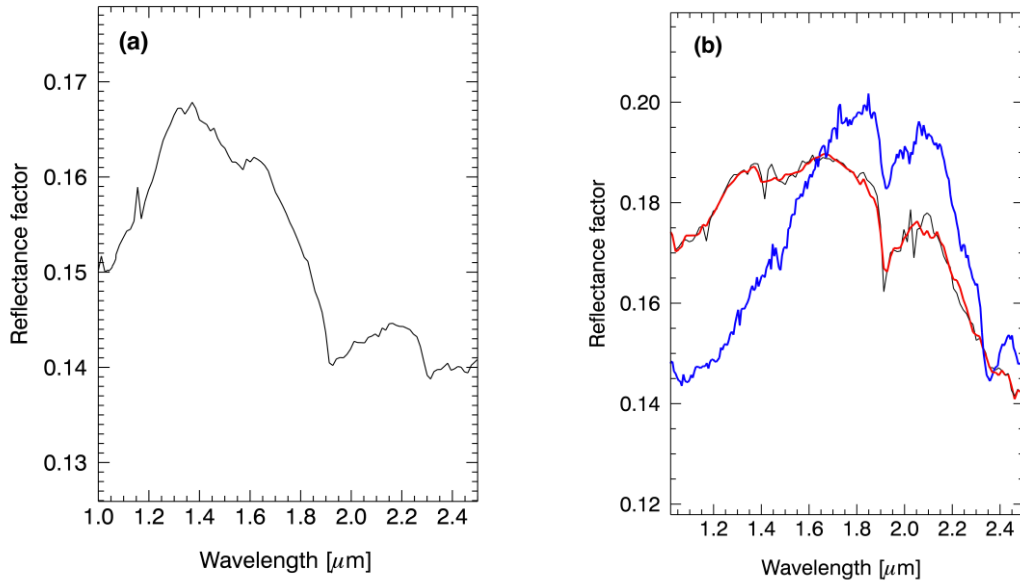
Figure 10. (a) Surface reflectance from orbit 0422_4 showing the absorption at 1.9 \mu\text{m} associated to 2.3 \mu\text{m} band indicating Fe/Mg-rich clays. (b) Surface reflectance factor showing the spectral feature of hydrated minerals at 1.9 \mu\text{m} , 2.3 \mu\text{m} and 1.4 \mu\text{m} in Nili Fossae region of Mars (MEX orbit 0422_4). The red line is the surface reflectance retrieved with the SAS procedure, the black line is the surface reflectance obtained with MO method, and the blue line is a CRISM observation of the same region but with a higher spatial resolution. The SAS method has not been applied to the CRISM spectrum in the figure, but the atmospheric features have been removed with “volcano scan” method (McGuire et al., 2009).
