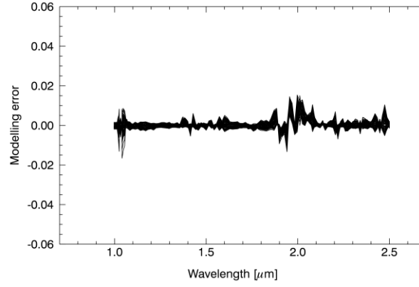
Figure 4. Modelling error computed as the difference between the true surface and the retrieved surface normalized to the true surface.
