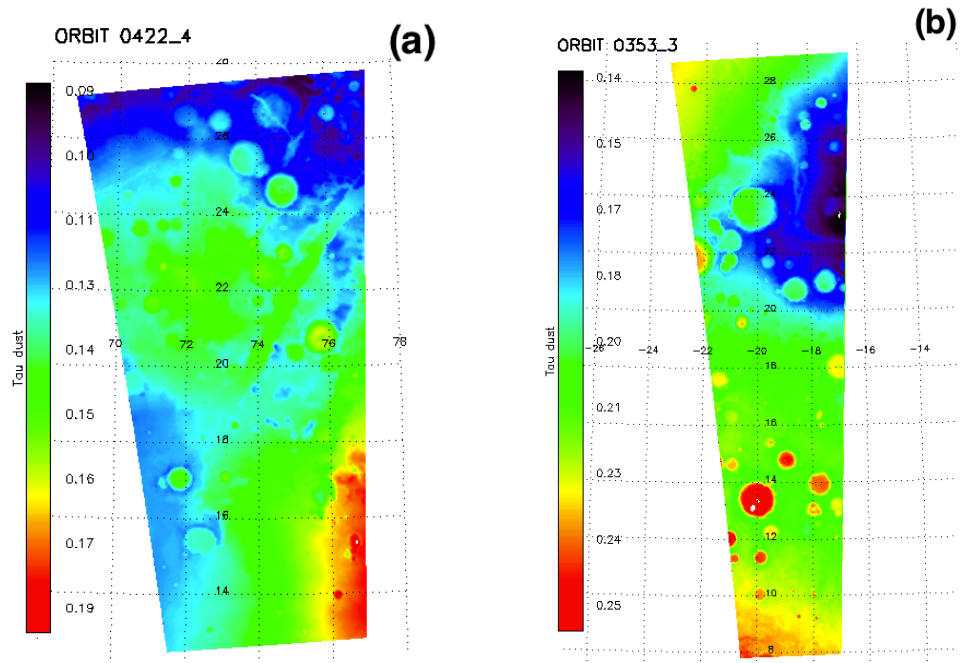
Figure 13. Maps of dust optical depth (at 1070\text{ cm}^{-1} ) as extracted from MCD. (a) Orbit 0422_4 and (b) orbit 0353_3.
