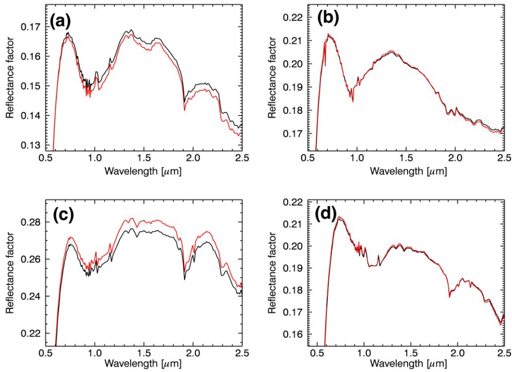
Figure 14. (a) Orbit 0422_4: pixel 75, scan 152. (b) Orbit 0422_4: pixel 77, scan 111. (c) Orbit 0353_3: pixel 41, scan 582. (d) Orbit 0353_3: pixel 38, scan 538. The black line is the surface reflectance and the red line is the surface reflectance corrected for the effect of dust in the atmosphere. The dust optical depths are 0.137 and 0.138 and 0.217 and 0.172 for the shown spectra of orbit 0422_4 and 0353_3, respectively.
