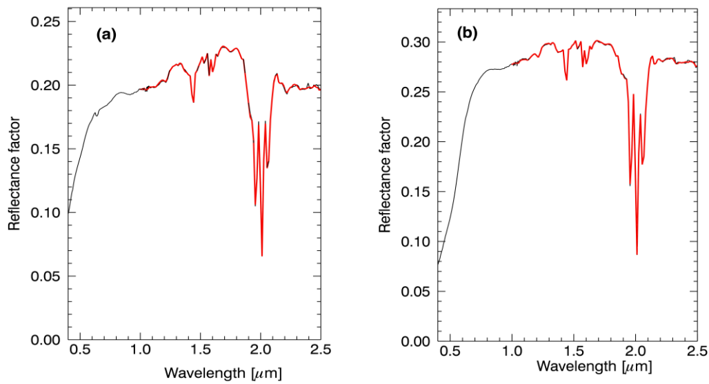
283 284 Figure 6. Reconstructed spectrum (red line) compared to the initial population (black line) for the same cases of Figure 285 5.
