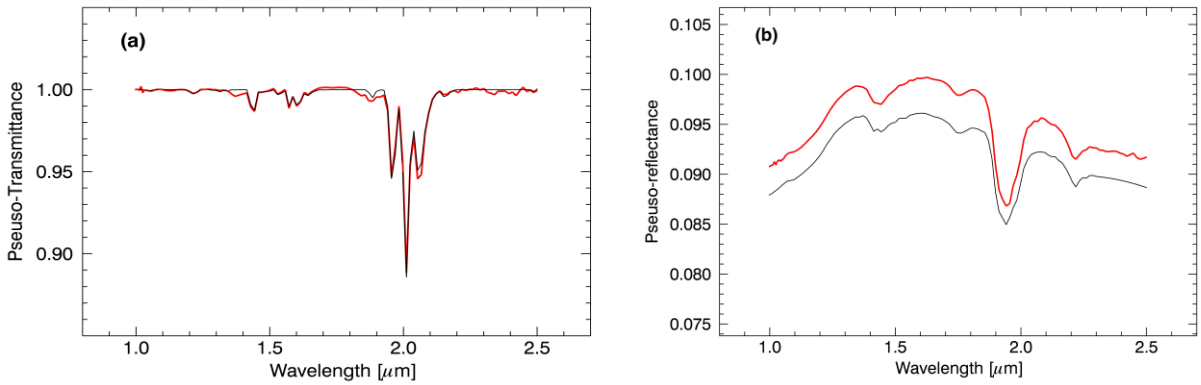
Figure 3. (a) Gas spectral component (red line) retrieved by fitting the trial spectra (black line) with a linear combination of significant eigenvectors. The gas trial spectrum (black line) is a simulated spectrum, which considers the contribution of carbon dioxide only. (b) Surface spectral component (red line, shifted for clarity) defined as the best-fit representation of trial spectrum (black line) with a linear combination of significant eigenvectors. The trial spectrum for the surface component (black line) is the linear combination of the dark and bright surface reflectance shown in Figure 1.
