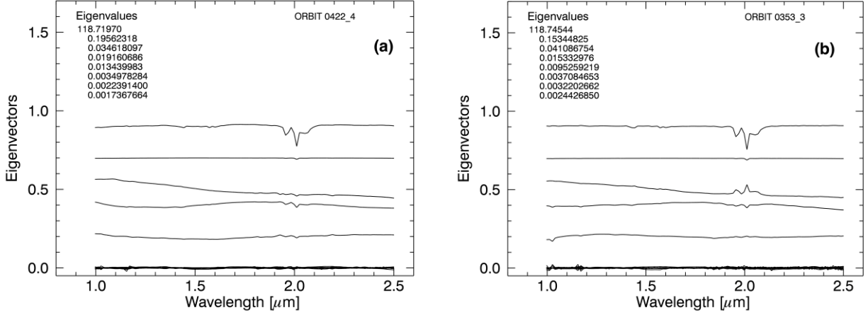
Figure 7. Eigenvectors (shifted for clarity) retrieved using PCA for the two considered orbits. Only the first eight eigenvalues are listed.
