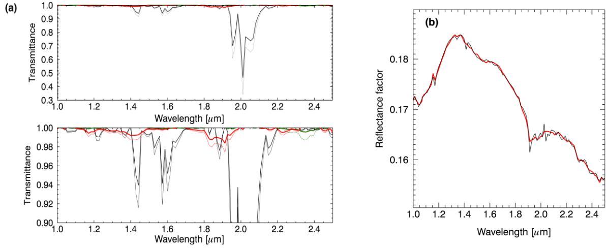
Figure 8. (a) Retrieved transmittances corresponding to the maximum (thick line) and minimum (thin line) weights. The CO 2 transmittances are the black lines, the H 2 O transmittances are the red lines and the CO transmittances are the green lines. The lower panel is a widening of the upper panel to have a better viewing of the CO and H 2 O transmittances. (b) Surface trial (black line) and retrieved surface end-member (red line) for a case where the hydrated band is present.
