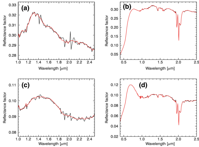
Figure 9. Spectra from orbit 0422_4 crossing bright and dark surfaces. (a and c) Surface reflectance factor retrieved using the methodology described in the paper (red spectra) overlying to surface reflectance obtained using MO method (black spectra). (b and d) Original OMEGA spectra (black line) underlying the retrieved spectra (red line) using the SAS procedure (red line).
