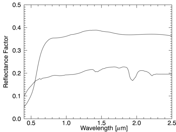
Figure 1. Reflectance of a bright surface (upper spectrum) and dark surface (lower spectrum) used as input for the surface reflectance in the RT code.
