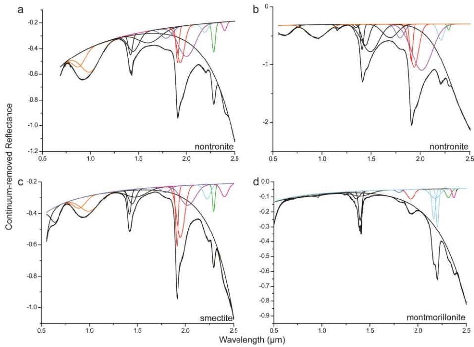
Fig. 15 MGM deconvolution on laboratory hydrated minerals: a,b) nontronites; c) smectite; d) montmorillonite. Spectra selected from the USGS spectral library are the black lines; the absorption contributions obtained with the MGM deconvolution are shown with colored lines.
