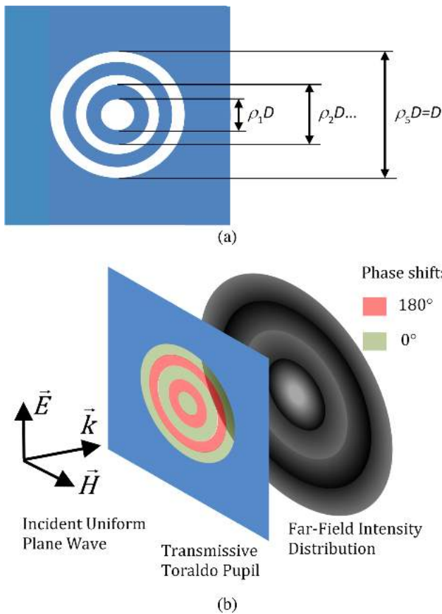
Fig. 1. Transmissive pupil structure: (a) conventional five-coronae transmissive pupil pattern with the shaded blue areas indicating opaque surface interspersed with transparent annular apertures; (b) Toraldo pupil structure with the transparent corona imparting alternate phase shift of 0^\circ (green) and 180^\circ (red) and the opaque area (blue) defining the outer diameter of the pupil.
