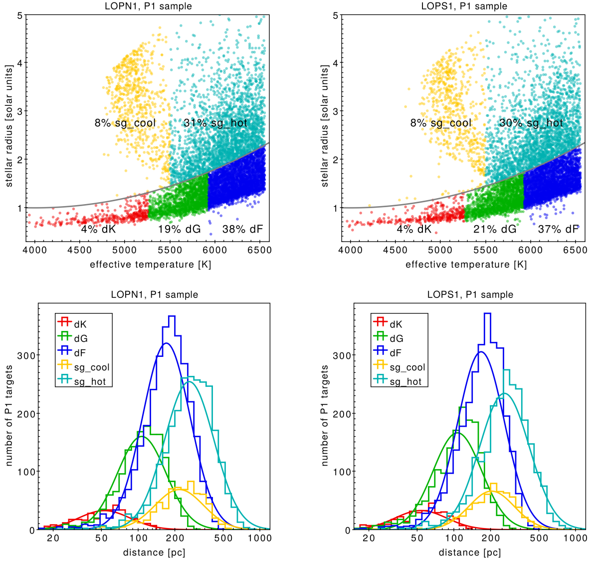
Fig. 9. Astrophysical parameters of the P1 targets within the LOPN1 (left panels) and LOPS1 (right panels) provisional fields. Top panels: Distribution of P1 targets on the (T_{\text{eff}}, R_*) plane; stars are classified into five distinct groups representing main-sequence K-type dwarfs (dK), G dwarfs (dG), F dwarfs (dF), subgiants at T_{\text{eff}} < 5500 K (sg_cool), and T_{\text{eff}} > 5500 K (sg_hot). The labels show their relative occurrence. The gray line in both panels marks an arbitrary boundary between main-sequence and evolved stars (see text). Bottom panels: Histograms of the distribution in distance of the same subgroups. The best-fit lognormal distribution is also over-plotted with a continuous line.
