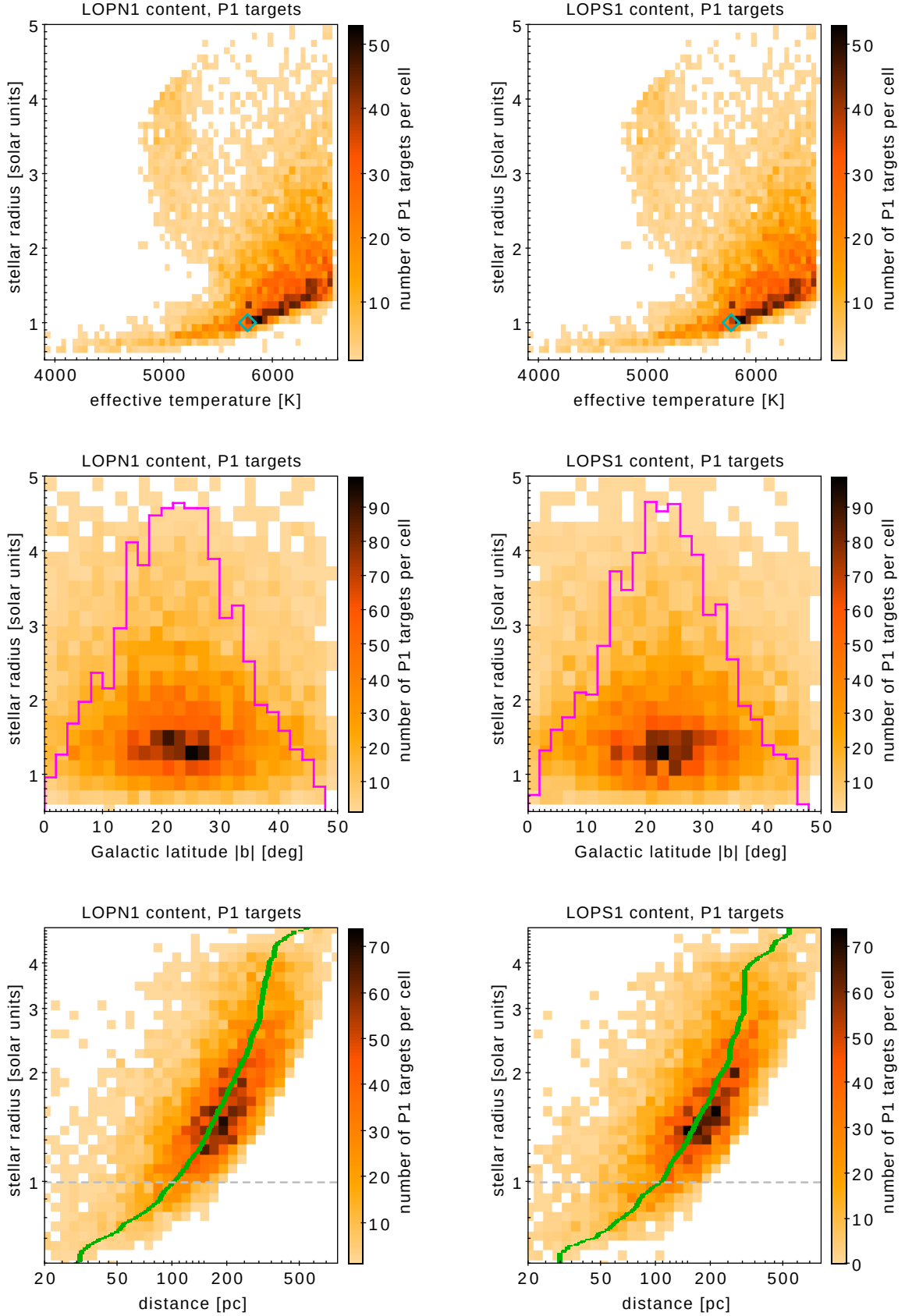
Fig. 8. Astrophysical parameters of the P1 targets within the LOPN1 (left panels) and LOPS1 (right panels) provisional fields. Top panels: Number density of P1 targets as a function of effective temperature and stellar radius. The high-density ridge corresponds to the main sequence, where the Solar parameters (1 R_{\odot} , 5778 K) are marked with a cyan diamond point as reference. Middle panels: Number density of P1 targets as a function of Galactic latitude |b| and stellar radius. A histogram of b is overplotted with a magenta line and arbitrary normalization. Bottom panels: Number density of P1 targets as a function of distance and stellar radius. The median distance at fixed solar radius is plotted with a green line.
