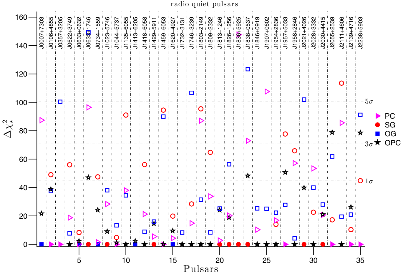
Fig. 3. Comparison of the relative goodness of the fit solutions obtained for the RQ LAT pulsars between the optimum-model and alternative models. The comparison is expressed as the \Delta\chi^2_* difference between the optimum and alternative model. The horizontal dash-dot lines indicate the confidence levels at which to reject a model solution compared to the optimum-solution. Triangles, circles, squares, and stars refer to the PC, SG, OG, and OPC models, respectively. Hereafter in all the figures of the paper, filled and empty symbols refer to the solutions of the optimum and alternative models, respectively.
