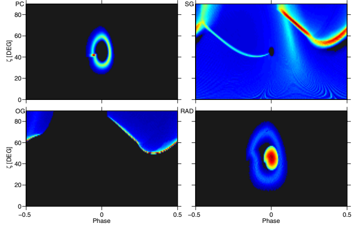
Fig. 1. Top left to bottom right panels: phase-plots obtained for the PC, SG, OG/OPC, and radio (core plus cone) models respectively, with a magnetic field strength of B_G = 10^8 Tesla and spin period of 30 ms for the PC and radio cases, and gap widths of 0.04 and 0.01 for the SG and OG/OPC cases, respectively. All the plots are given for an obliquity \alpha = 45^\circ . The emission flux increases from black to red.
