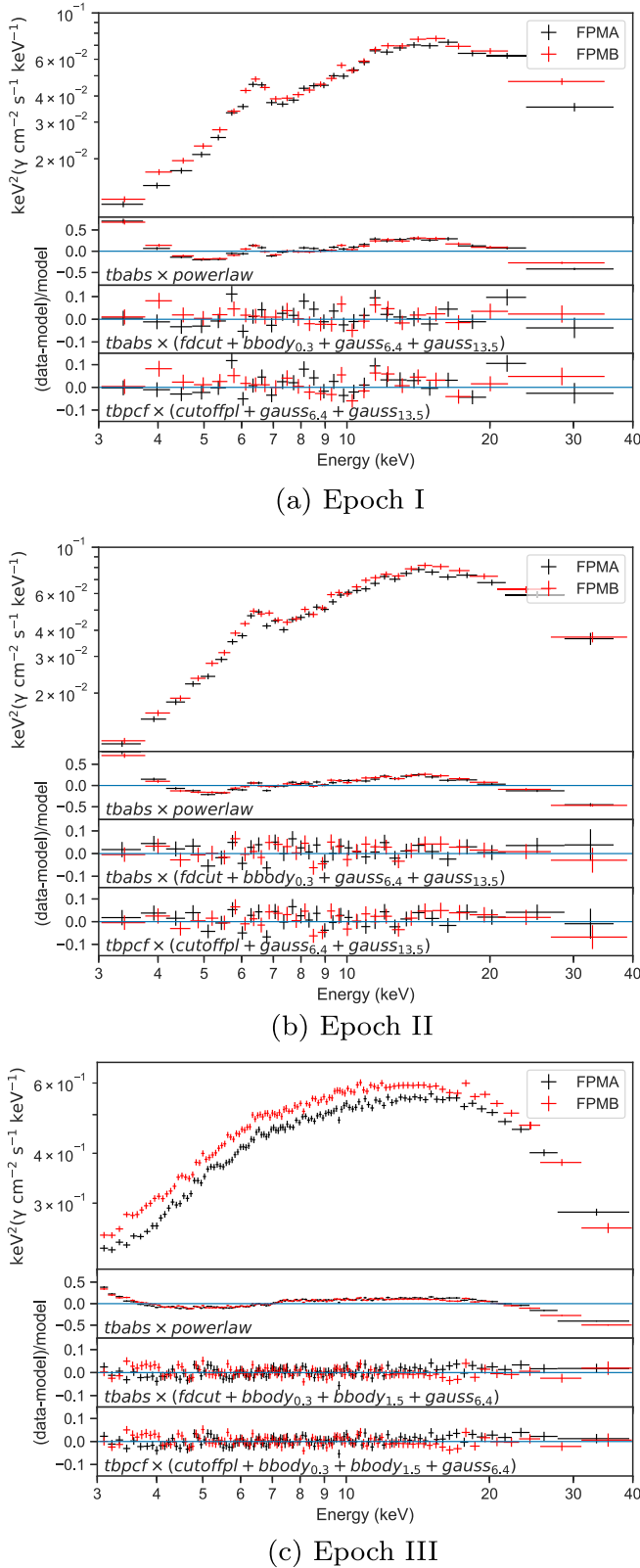
Figure 4. Observed spectra for each epoch are shown unfolded against a model with constant (energy-independent) flux in the top panels, and fitting residuals for three different models are shown in the lower panels. The FPMA spectra are shown in black while the FPMB spectra are shown in red. The data is consistently described well by a partially absorbed power law with a high energy cutoff. While the shape of the continuum remains relatively constant, the covering fraction and absorbing column vary between successive epochs, with the covering fraction decreasing significantly between Epoch II and Epoch III.
