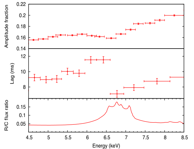
Figure 3. Amplitude fraction (upper panel) and phase delay (middle panel) of the fundamental harmonic as function of energy in the 4.5–8.5 keV energy range. Ratio of the fluxes from the reflected and the irradiating continuum (lower panel), according to the spectral decomposition in D’Ai et al. (2015).
