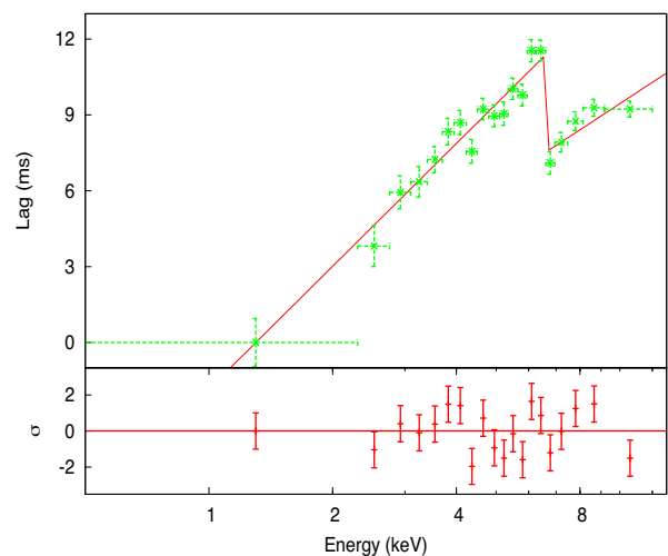
Figure 4. Best-fitting piecewise function [equation (2), with a break at 6.6 keV] of the EPIC/pn data (Fig. 1) and residuals in units of \sigma (lower panel).
