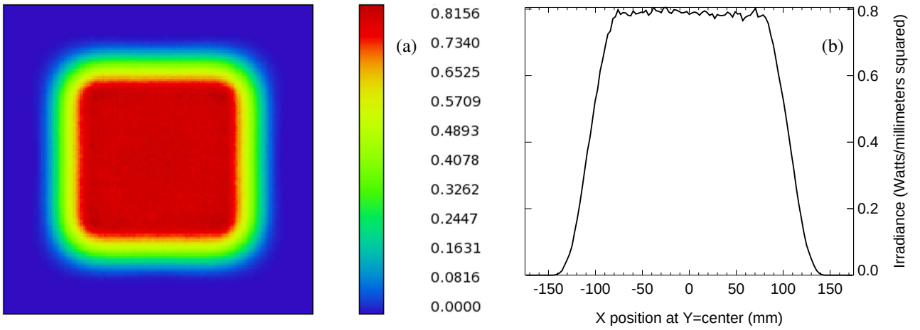
Figure 6: a) 2D and b) x-cross section irradiance produced by the optics coupled to the type-3 designed for 800 \times . The physical size of the figures is 350 mm. Units in the color bar are \text{Watt/mm}^2 .
