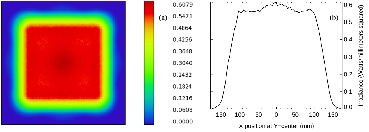
Figure 5: a) 2D and b) x-cross section irradiance produced by the optics coupled to the type-3 designed for 500 \times . The physical size of the figures is 350 mm. Units in the color bar are \text{Watt/mm}^2 .
