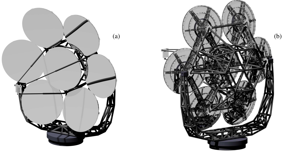
Figure 7: Shaded models of the SOLARIS Concentrator: a) front side, b) rear side.
