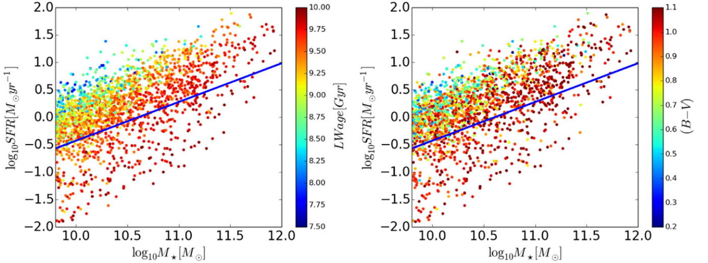
Figure 4. SFR– M_* relation for cluster galaxies. The slanted solid blue line shows the limit dividing PSF and transition galaxies. Color-coded are the luminosity-weighted age (left) and (B - V) color (right).
