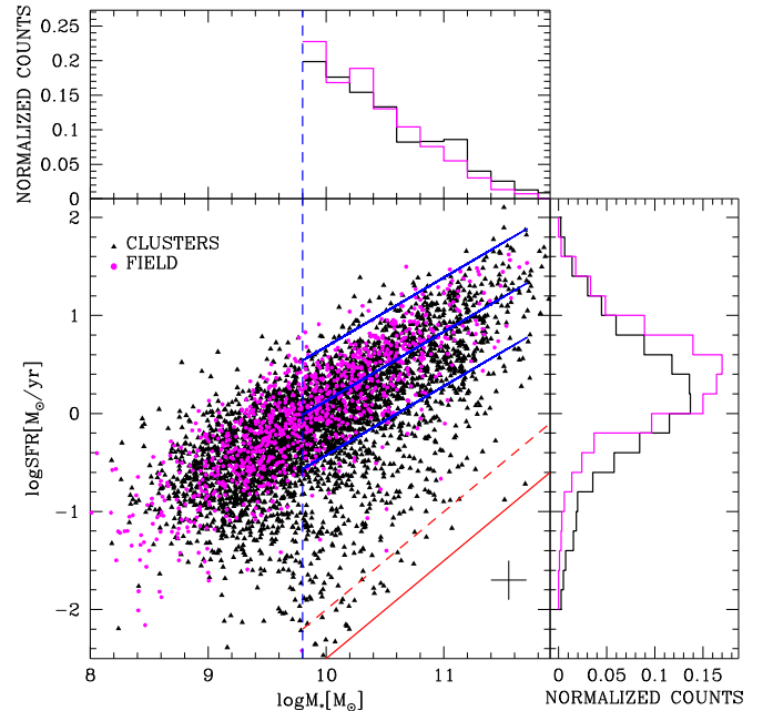
Figure 1. Main panel: SFR– M_* relation for cluster (black triangles) and field (magenta circles) galaxies. The blue solid lines indicate the best fit of the field with 1.5\sigma error, the red solid (dashed) line the \log \text{sSFR} = -12.5 ( -12 ) limit. The blue vertical dashed line indicates the mass completeness limit. Typical error bars on SFR and M_* are indicated in the bottom right corner. Upper panel: cluster (black) and field (magenta) mass distributions. Right panel: cluster and field SFR distributions above the mass completeness limit. Histograms are normalized to total and weighted for incompleteness.
