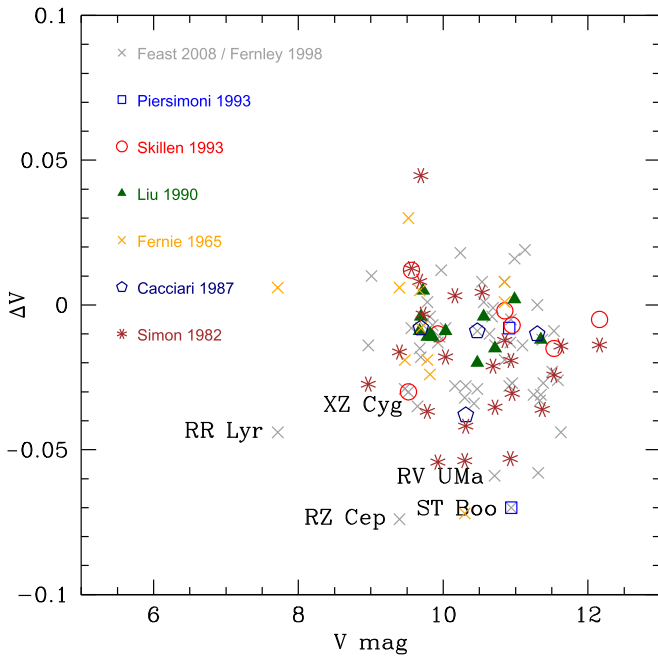
Figure 5. Difference between the current intensity mean values \langle V \rangle and values published in the literature as described in the text.
