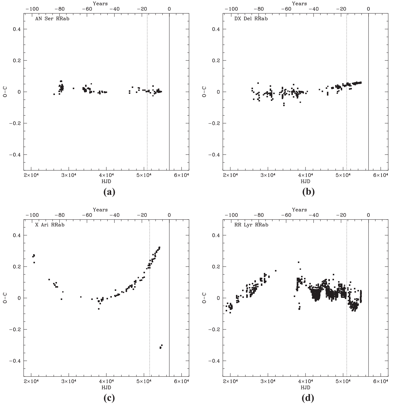
Figure 3. Data from GEOS (Section 4.1.2) demonstrating phasing solutions in the O–C diagram (see Section 5.1 for details) for the four cases described in the text. The solid vertical line highlights the epoch of the TMMT data and the dashed vertical line is at the epoch of the 2MASS observations. (a) Flat O–C behavior (for AN Ser) implies that no updates to period are required. (b) Linear O–C behavior over the last 30 years (for DX Del) implies that the period is slightly longer than originally determined. (c) Quadratic O–C behavior (for X Ari) implies that the period itself has been changing over time. (d) Chaotic O–C behavior (for RR Lyr) implies that neither adding precision to the period nor applying a shift in period is sufficient to phase all of the individual data sets analytically. In this case, each data set gets a custom phase offset for alignment to the current TMMT epoch.
