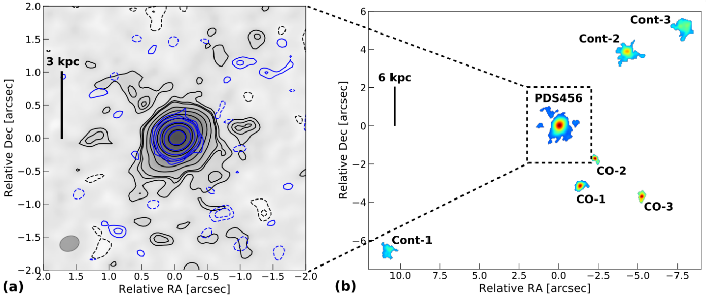
Fig. 1. Panel (a): map of the continuum-subtracted, CO(3–2) emission of PDS 456 integrated over a linewidth of 320 \text{ km s}^{-1} . Black contours indicate the [-3, -2, 2, 3, 2']\sigma significance levels ( n \geq 2 and \sigma = 0.013 \text{ Jy beam}^{-1} \text{ km s}^{-1} ) of the CO(3–2) emission. Blue contours indicate the (rest-frame) \sim 340 \text{ GHz} continuum [-3, -2, 2, 3, 2']\sigma levels (with \sigma = 9.6 \mu\text{Jy beam}^{-1} ). The ALMA synthetic beam is indicated by the grey ellipse. Panel (b): map of the line and continuum emitters detected in the ALMA field of view at \geq 5\sigma .
