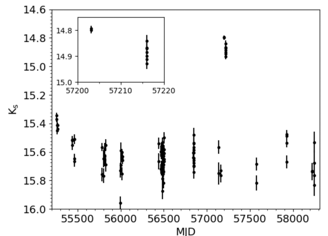
Figure A1. VVV K_s light curve for the submm-bright source VVV J161053.93-515532.8. A jump of \sim 0.9 mag occurred in mid-2015, lasting for at least 13 d. The flux had returned to the pre-outburst level in data taken 12 months later. The inset panel shows an expanded view of the data during the outburst.
