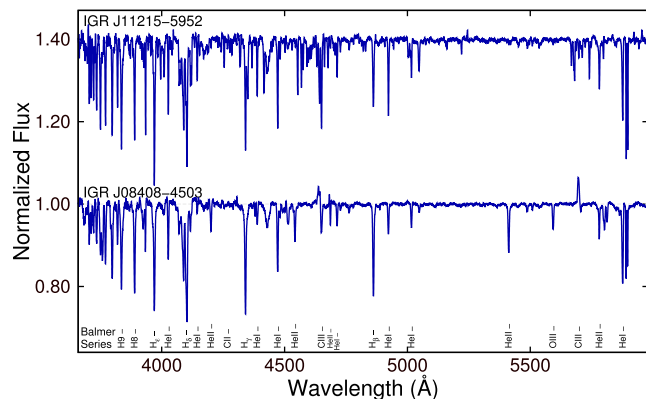
Figure 1. Normalized FORS 2 Stokes I spectra of IGR J08408–4503 and IGR J11215–5952. Well-known spectral lines are indicated at the bottom. The spectrum of IGR J11215–5952 was vertically offset by 0.4 for clarity.
