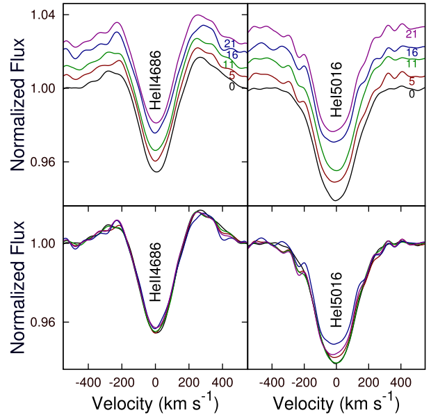
Figure 7. The behaviour of He II 4686 and He I 5016 in the spectra of IGR J08408–4503 obtained for individual sub-exposures belonging to the observation on 2016 December 5. In the upper row, we present the line profiles shifted in vertical direction for best visibility. The time difference (in minutes) between each sub-exposure and the start of observations is given close to each profile. The lower row shows all profiles overplotted.
