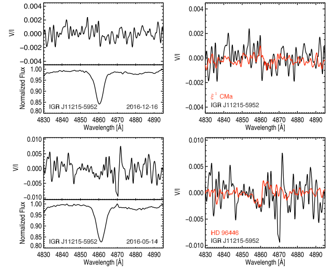
Figure 4. Left-hand panel: Stokes V and Stokes I spectra of IGR J11215–5952 in the spectral region around the H\beta line at two different epochs. Right-hand panel: Stokes V spectra of IGR J11215–5952 are overplotted with the Stokes V spectra of the two well-known magnetic early-B type stars \xi^1 CMa ( \langle B_z \rangle_{\text{hydr}} = 360 \pm 49 G) and HD 96446 ( \langle B_z \rangle_{\text{hydr}} = -1590 \pm 74 G) for best visibility of the Zeeman features.
