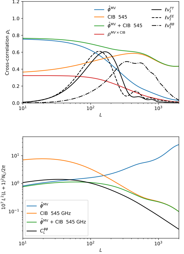
Fig. 11. Top: Expected cross-correlation coefficient of the true lensing potential to the minimum-variance (MV) estimator, the 545-GHz GNILC CIB map (orange), and their combination (green). To build these curves, the cross-spectrum of the CIB map to the true lensing potential is approximated by its cross-spectrum to the MV (quadratic-estimator) lensing reconstruction, displayed in Fig. 10, and GNILC CIB curves are smooth spline fits. The red curve shows for comparison the cross-correlation coefficient of the CIB to the MV quadratic estimator. This cross-correlation is suppressed by instrument noise, foreground residuals, and shot noise in the CIB map and reconstruction noise in the lensing quadratic estimator. The black curves show the lensing kernels that contribute to the lensing of the temperature (solid), E -mode polarization (dashed), and B -mode polarization (dash-dotted) power spectra, as described in the text. Bottom: Effective reconstruction noise levels N_L for each of these tracers, as defined by Eq. (48), and, for comparison, the theoretical lensing spectrum C_L^{\phi\phi} . The quadratic estimator reconstruction noise is slightly underestimated at low L in this figure, since we have neglected Monte Carlo corrections when combining the tracers.
