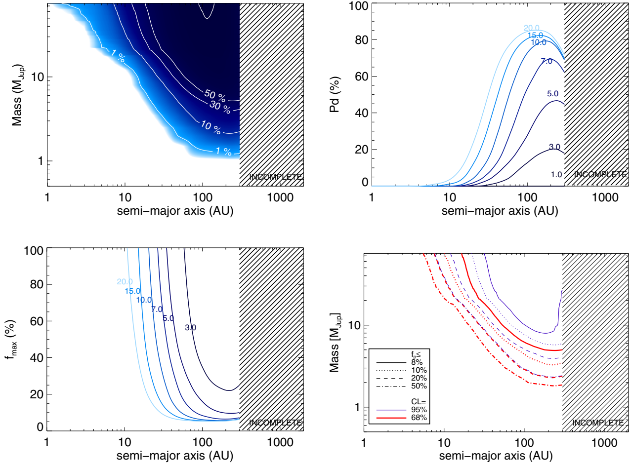
Fig. 8. Results for the complete-stat sample. Top left: NaCo-LP mean detection probability map ( \langle p_i \rangle ) as a function of the mass and semi-major axis. Top right: mean probability curves for different masses (1, 3, 5, 7, 10, 15, and 20 M_{\text{Jup}} ) as a function of the semi-major axis. Bottom left: giant planet and brown dwarf occurrence upper limit ( f_{\text{max}} ), considering a 95% confidence level, for different masses (3, 5, 7, 10, 15, and 20 M_{\text{Jup}} ) as a function of the semi-major axis considering the null-detection result and an uniform distribution of planets and brown dwarfs in terms of masses and semi-major axis. Bottom right: same occurrence upper limit ( f_{\text{max}} ) expressed this time in a mass versus semi-major axis diagramme for a 68% and 95% confidence level (following Biller et al. 2007; Nielsen et al. 2008 representation).
