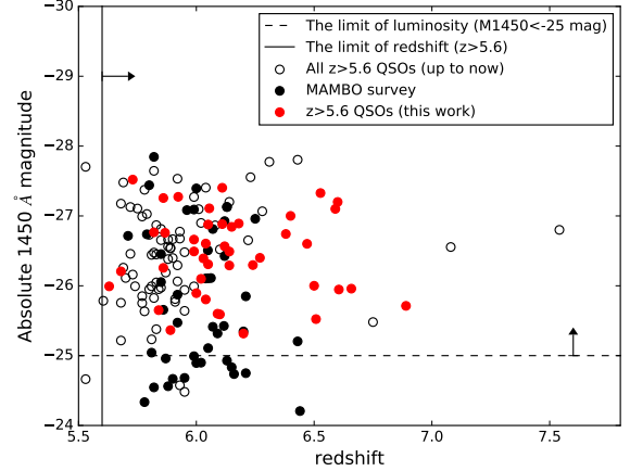
Figure 1. The sample selected from available quasar surveys before our observations. More than 250 quasars at z > 5.6 are known today (all circles). The red circles indicate the sources which belong to the sample in SHERRY, see Section 2.1.
