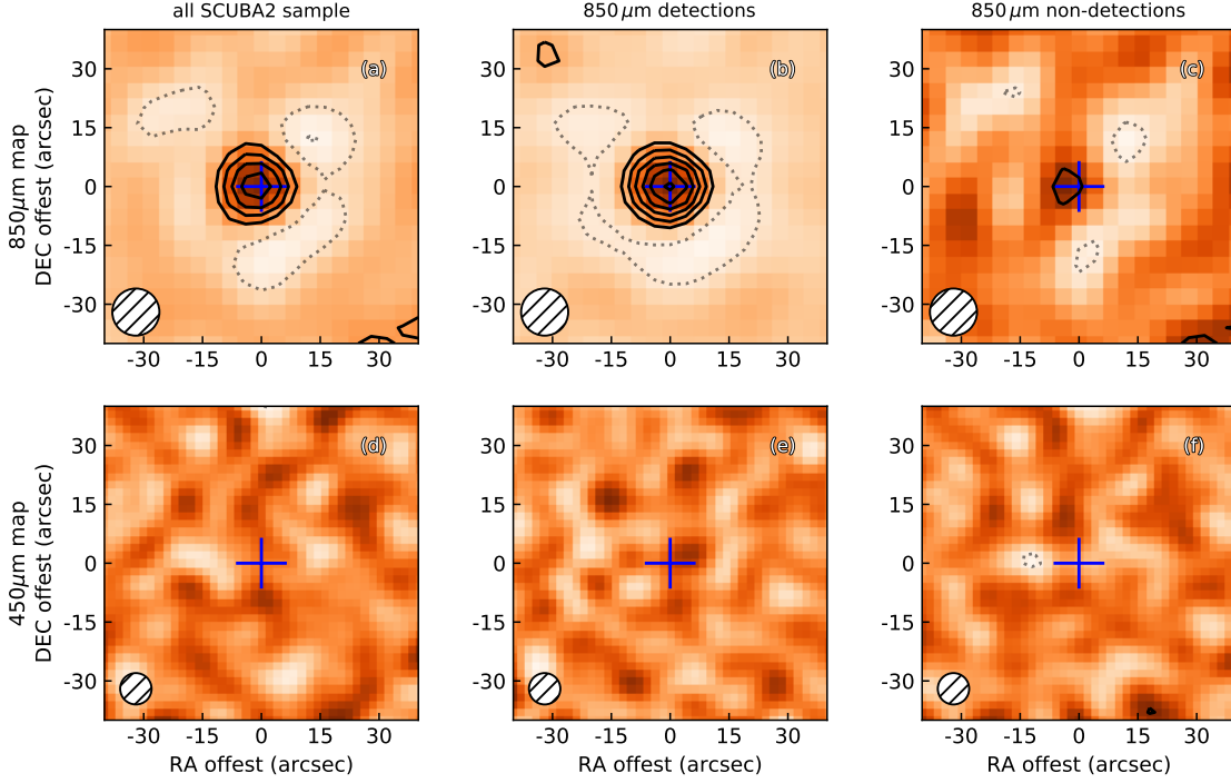
Figure 3. 80 \times 80 \text{ arcsec}^2 SCUBA2 850 \mu\text{m} and 450 \mu\text{m} stacked maps of (a, d) all the SHERRY sample, (b, e) 850 \mu\text{m} detections and (c, f) 850 \mu\text{m} non-detections. The blue cross denotes the quasar optical position. The white circle shows the SCUBA2 beam size at 850 \mu\text{m} of 15'' and at 450 \mu\text{m} of 7''.9 . The colour scale in \text{mJy beam}^{-1} goes from white to orange with the contour levels of [-6, -3] and [+3, 6, 9...]\times\sigma (dotted and solid lines). The stacking procedure used to produce this image is described in Section 3.2.
