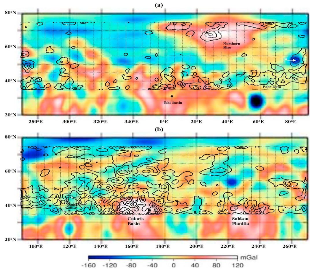
Figure 5. As in Figure 4 but superposed onto a MESSENGER radio tracking free-air gravity anomaly map (A. Genova, private communication, 2018).
