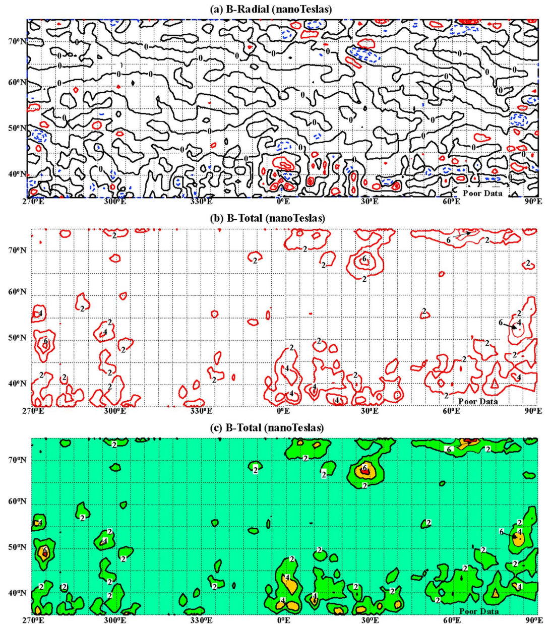
Figure 2. Equivalent source dipole modeling results: (a) radial magnetic field component at 40-km altitude calculated from the equivalent source dipole solution; (b) magnetic field magnitude at 40 km (contour interval, 2 nT); (c) as in (b) but shaded to emphasize stronger anomalies. The contour interval and color scheme for the radial field map are the same as in Figure 1.
