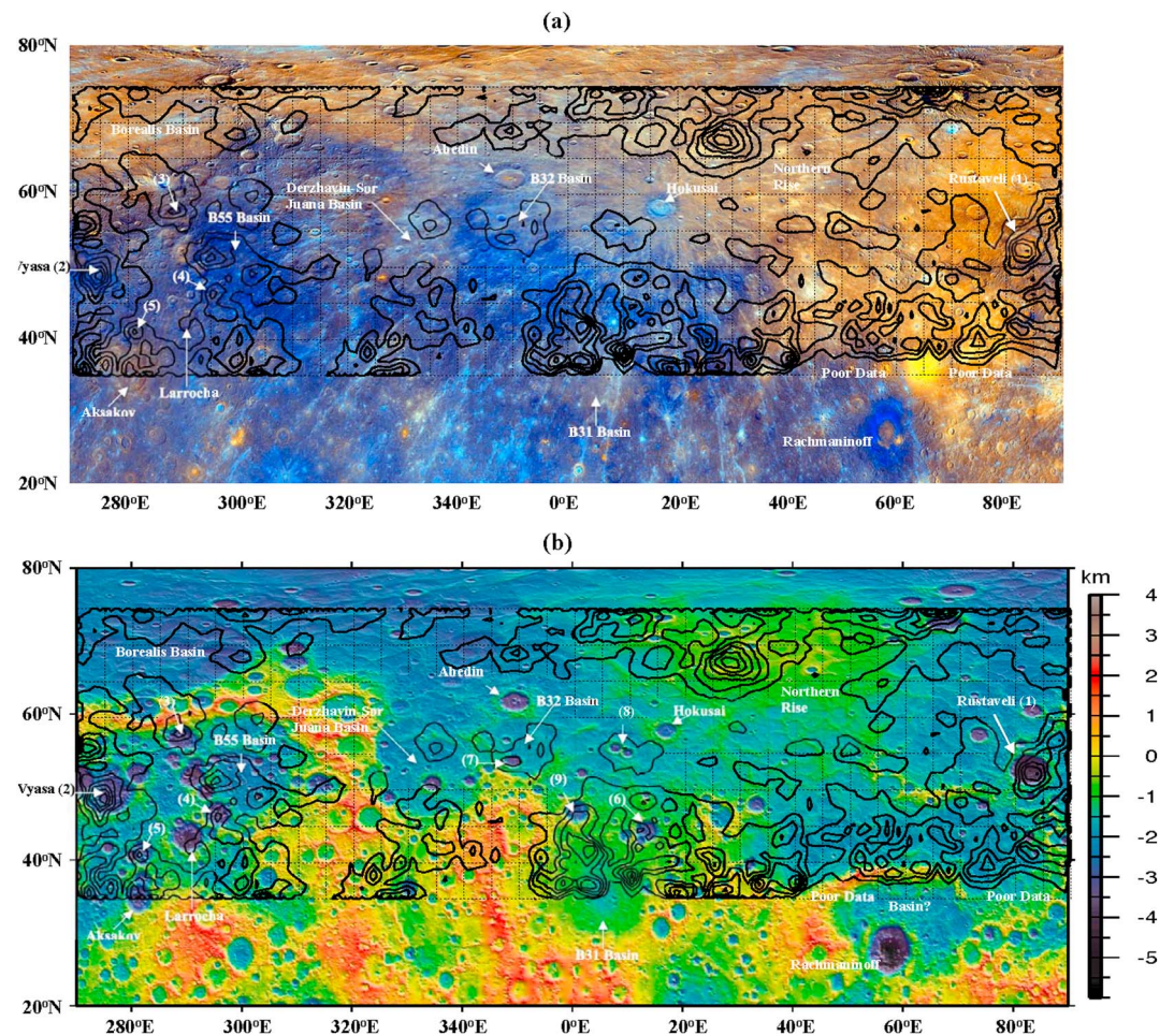
Figure 3. Superposition of the equivalent source dipole field magnitude at 40-km altitude (contour interval, 1 nT) onto: (a) a MESSENGER enhanced color image composite; and (b) a Mercury Surface, Space ENvironment, GEochemistry, and Ranging Laser Altimeter elevation map. See the text for further explanation.
