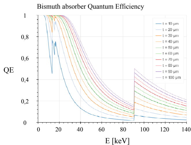
Figure 2 – QE of bismuth absorbers with different thickness, based on X-ray absorption data 19 .
