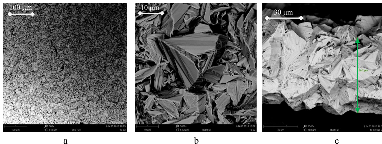
Figure 8 – Electroplated bismuth layer SEM micrographs: low magnification (a); high magnification (b); lateral view with about 67\ \mu\text{m} measured thickness evidenced (c).
