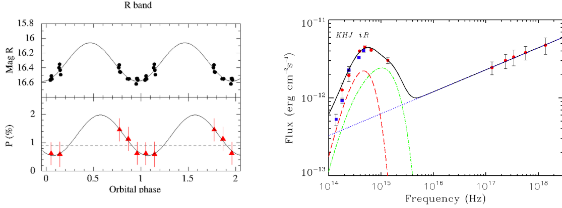
Figure 2. Left panel, up: R -band light curve of J1023 (magnitude vs. orbital phase). With a solid line, a fit of the light curve with a sinusoidal function with period fixed to 1 (corresponding to 4.75 hr) is reported. The \chi^2/\text{dof} of the fit is 11.35/17; bottom: R -band polarisation curve represented with respect to the orbital phase of the system. Superimposed, the fits with a constant function (dashed line; \chi^2/\text{dof} = 3.66/4 ) and with a sinusoidal function with period fixed to 1 (solid line; \chi^2/\text{dof} = 0.11/2 ). Errors are represented at the 68% confidence level. Two periods are drawn for clarity. Right panel: NIR–optical contemporaneous SED of J1023 obtained in this work (orbital phase 0.59; blue squares); the NIR–X-rays SED of J1023 reported in [23] is also represented (red dots), with superimposed the fit with a model made by the companion star (red dashed line), the accretion disc (green dash-dotted line) and the shock emission powered by the neutron star (NS) spin down luminosity (blue dotted line).
