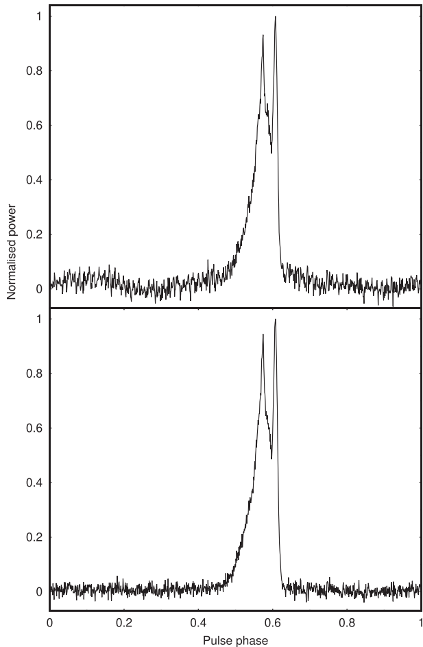
Figure 7. The pulse profile of PSR J1022+1001, folded over 60 min of a LEAP observation with a bandwidth of 128 MHz, both without (top) and with (bottom) interference removal using spectral kurtosis. Both panels show the contribution from the Nançay radio telescope only, with spectral kurtosis applied using M = 1000 , N = 2 , and \eta = 3 , and rejected data replaced by artificial Gaussian noise. While zapping of the folded observation is ineffective at removing this interference, spectral kurtosis improves the estimated accuracy of the pulse arrival time measured at Nançay from 1.22 to 0.70 \mu\text{s} .
