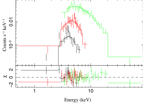
Figure 2. NuSTAR FPMA and FPMB combined spectra (green) and Chandra zeroth-order and 1 st order spectra (black and red, respectively) for flare Nu6 peak jointly fitted to an absorbed power-law model. The crosses show the data points with 1- \sigma error bars, and the solid lines show the best fit model. The lower panel shows the deviation from the model in units of standard deviation.
