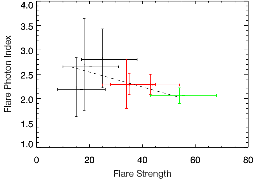
Figure 3. Spectral Index vs. strength for seven NuSTAR X-ray flares with detection significance > 5\sigma (with 90% error bars). The flare strength is defined as the ratio of the flare 2–10 keV unabsorbed flux and the quiescent state flux of F_q(2-10 \text{ keV}) = 0.47^{+0.04}_{-0.03} \times 10^{-12} \text{ erg cm}^{-2} \text{ s}^{-1} . The seven flares are grouped into three sets: flares with flare strengths less than 30 times the Sgr A* quiescent flux: Nu1, Nu2 and Nu9 in black; flares with strengths higher than 30 times but lower than 50 times the Sgr A* quiescent flux: Nu3, Nu7 and Nu8 in red; and flares with strengths higher than 50 times the Sgr A* quiescent flux: Nu6 in green. A linear fitting of the flare indices over strengths (with 90% error bars considered) gives a slope of a = -0.016 \pm 0.010 , suggesting no significant correlation between the flare spectral shape and the flare luminosity.
