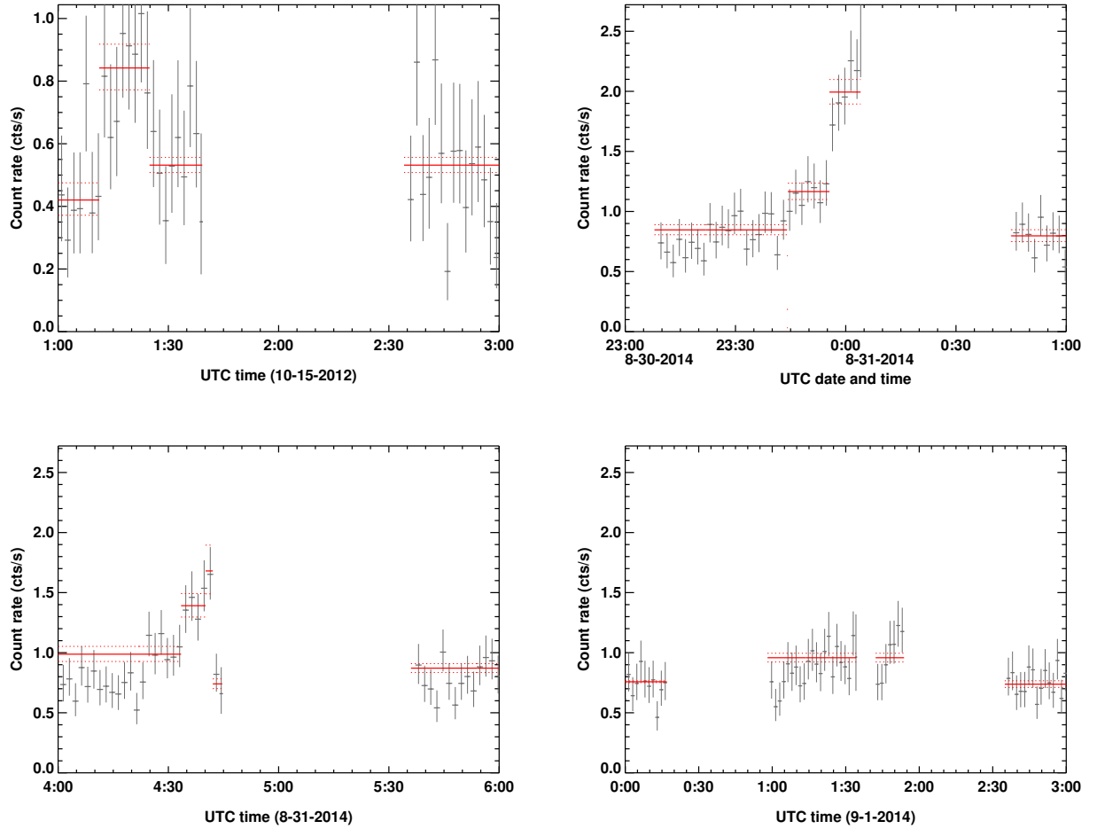
Figure 1. NuSTAR 3 – 79 keV light curves showing previously unreported flares with > 3\sigma detections, including flare Nu5 (upper left), Nu7 (upper right), Nu8 (lower left) and Nu9 (lower right). The NuSTAR light curves are deadtime, PSF, and vignetting corrected and extracted from a 30'' radius circle centered on Sgr A* in 100s bin. The light curves of the four bright flares Nu1, Nu2, Nu3 and Nu6 are shown in Figure 1 and 2 in Barrière et al. (2014). Flares Nu4 and Nu10 are not significantly detected with NuSTAR data only. The Nu4 Chandra light curve is presented in Neilsen et al. (2013); the Nu10 XMM-Newton light curve is presented in Ponti et al. (2015).
