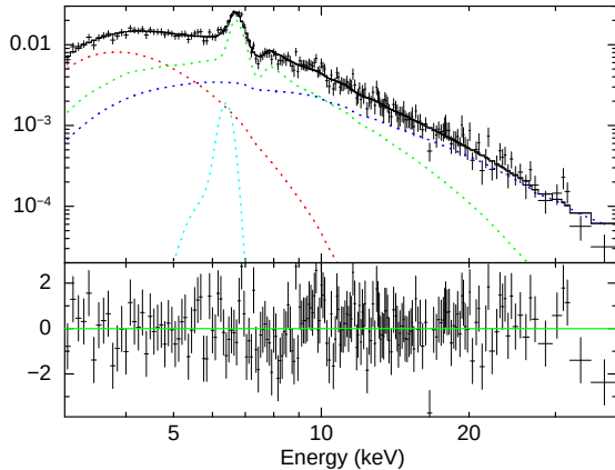
Figure 4. NuSTAR FPMA spectrum for the inner 30'' of the Sgr A* region during its X-ray quiescence with the best-fit model. The spectrum is well-fit with a multi-component model with individual components in different colors: two apec models with kT_1 \sim 1.1 keV (red) and kT_2 \sim 6.7 keV (green), a Gaussian for 6.4 keV neutral Fe line (cyan) and a power-law (blue), resulting in \text{tbabs}^*(\text{apec1}+\text{apec2}+\text{gaussian}+\text{power-law}) . The thermal apec components become negligible above 20 keV, where the non-thermal power-law component starts to dominate. This spectrum can help to constrain the Sgr A* quiescent luminosity level, though it is likely dominated by a PWN candidate and diffuse X-ray emission.
