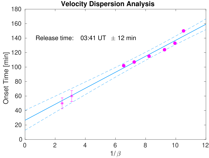
Figure 10. The behavior of the observed onset times and the inverse velocities, 1/\beta . Filled dots refer to STEREO-B/LET observations in the energy range 4–12 MeV, while asterisks refer to the highest-energy channels of STEREO-B/HET (i.e., 40–60 MeV and 60–100 MeV, respectively). The solid line depicts the best fit according to Equation (1), while the dashed lines are the 95% confidence levels. The release time, given on the top-left corner of the figure, is obtained as the intercept of the best-fit line with the y-axis and it is given in minutes after the solar flare.
