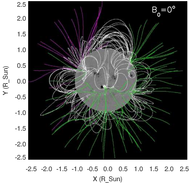
Figure 14. The extrapolated coronal magnetic field as obtained by the PFSS model from the photospheric magnetic field measured by SDO/HMI for B_0 = 0 , where the Earth is orthogonal to the figure. White lines correspond to closed magnetic field lines; violet and green lines represent open incoming (negative polarity) and outgoing (positive polarity) magnetic field lines, respectively.
