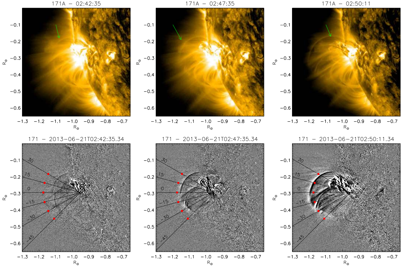
Figure 3. The expanding EUV front as seen through the SDO/AIA 171 Å passband (top panels) and the corresponding RD images (bottom panels) at three different times: 02:42, 02:47, and 02:50 UT, respectively, over a 0.65 \times 0.65 R_\odot region. Red dots indicate regions where intensities were calculated, at different inclination angles with respect to the eruption foot-point. The green arrow highlights the expanding front.
