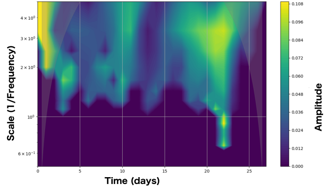
Figure 6. Wavelet analysis of the XRT PC data shows no period but bursty behaviour. The Y-axis shows the time-scales (in days) searched for.
