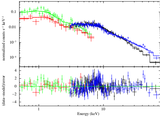
Figure 5. The combined XRT and NuSTAR spectra fit. The first NuSTAR observation (blue) and the 2nd NuSTAR observation (black) are shown with their XRT counterparts (green and red respectively).
