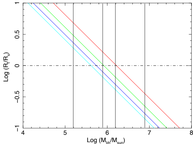
Figure 9. Constraints to the systems parameters for a tidal disruption event in a \log(R_t/R_s) vs \log(M_{\text{bh}}/M_{\odot}) plot, where M_{\text{bh}} is the black hole mass and R_s is the Schwarzschild radius. The inclined coloured lines correspond to the tidal disruption radii for helium white dwarfs of masses 0.1, 0.2, 0.3 and 0.4 M_{\odot} (from top to bottom respectively). Tidal disruption is allowed when R_t > R_s , and the critical condition where R_t = R_s is indicated by the dotted-dashed horizontal line. The vertical lines indicate the lower bounds of the black hole masses for the parameters \eta\zeta = 5, 1, 0.5 and 0.1 (from left to right respectively).
