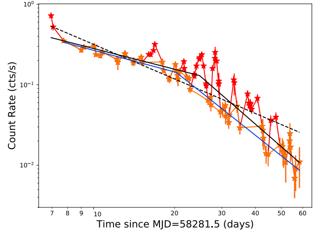
Figure 4. A log-log plot of the XRT light curve indicates that the evolution of the X-ray emission follows a broken power-law with a break at day T_d+21 . Three fits are shown: fitting all data with a single PL (black dashed line), or with a broken PL (black line) as well as a fit to the data excluding obvious flaring points (blue line). The flaring points which are shown here in red.
