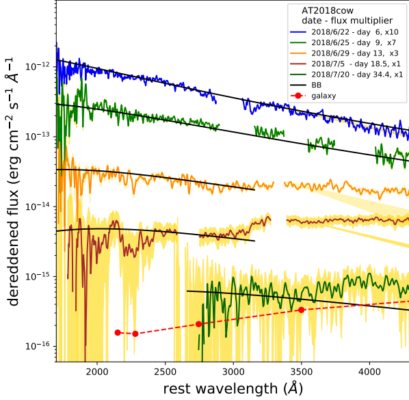
Figure 3. The dereddened UVOT grism spectra, using E(B-V) = 0.077 and the Cardelli et al. (1989) law with R_V = 3.1 . The 1\sigma errors are indicated with shading. The features below 2200 \text{ \AA} are due to noise. Black-body fits are included, as well as the galaxy brightness in the 3'' radius aperture used for photometry. Excess flux on day T_d+13 and 18.5 longer than 3000 \text{ \AA} is due to order overlap.
