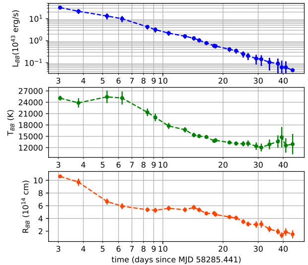
Figure 2. Black-body model fit to the UVOT data in a log-log plot. Note that the luminosity decays approximately as a power law with different slopes before and after day T_d+6.5 . After day T_d+44 the galaxy background emission in v and b do no longer allow a good fit to be made.
