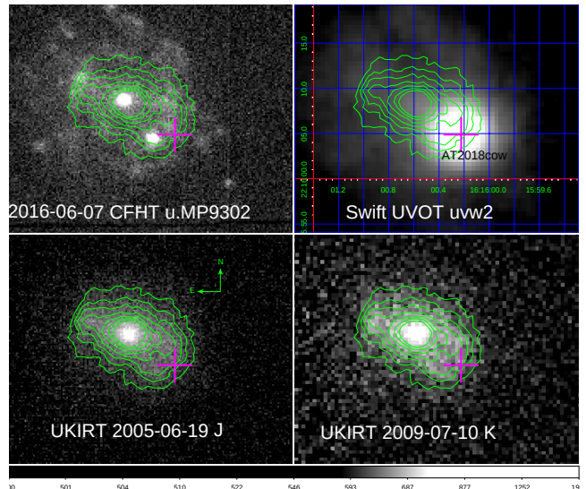
Figure 12. Galaxy Z 137-068 in pre-explosion u (CFHT), J , and K (UKIDSS) and after explosion Swift uvw2 image with AT2018cow position indicated by a cross. Contours are taken from the J -band image and superimposed on the others. The IR images in J and K show to the south-west extra emission that breaks the overall symmetry of the galaxy. The u band image shows near the extra South-West emission a strong UV bright source. In the u band many small small clusters of bright emission can be seen around the galaxy contour.
