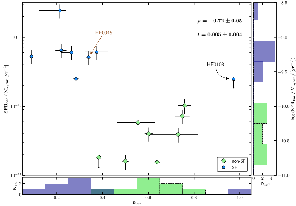
Fig. 7. Comparison between the sSFR and the Sérsic index of the bar. The s_{\text{SFR}}_{\text{bar}} is the SFR normalised by the stellar mass of the bar in the intermediate bar region that includes the rows -3 to -1 and 1 to 3 as defined in Fig. 5. The index n_{\text{bar}} is the Sérsic index of the main bar component bar1 . The objects are divided into non-SF (green) and SF (blue) according to the classification in Fig. 6. Bottom and right panels: histograms for both parameters. There is a clear separation in \log(s_{\text{SFR}}_{\text{bar}}) as we have seen before. The separation is also apparent in n_{\text{bar}} with only marginal overlap. The galaxy HE 0108–4743 annotated in black is discussed separately in the text. HE 0045–2145 (indicated with a brown arrow) is the only galaxy not hosting an AGN in the sample. The error bars for n_{\text{bar}} show the 68% confidence intervals from the posterior distribution of our bootstrap resampling method. More details about the uncertainties can be found in the main text and Appendix A.1. In the top right corner, we show the Spearman’s rank correlation coefficient \rho and the t -value for a null-hypothesis test.
