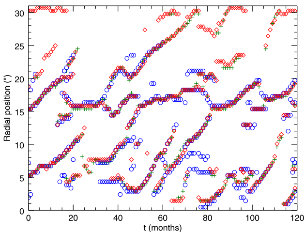
Figure 3. Radial position of local intensity maxima (in arcseconds) as a function of time (in months) referring to case (1) (i.e. uniform injection). Red diamonds are for radio emission, green crosses for optical and blue circles for the X-rays.
