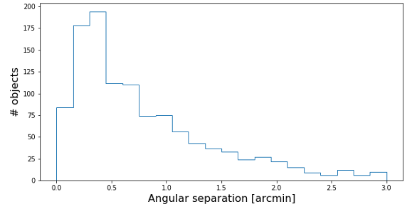
Figure 1. Distribution of angular separations between ALMA and Planck Collaboration XXVI (2016) positions of the 1,120 sources resulting from the cross-match ( 3' search radius) between the ACC and the PCNT catalogues.
