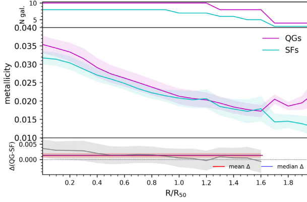
Figure 14. The average radial profiles of the gas-phase metallicity Z for QG and SF samples. The layout of the figure is the same as in Fig. 10.
