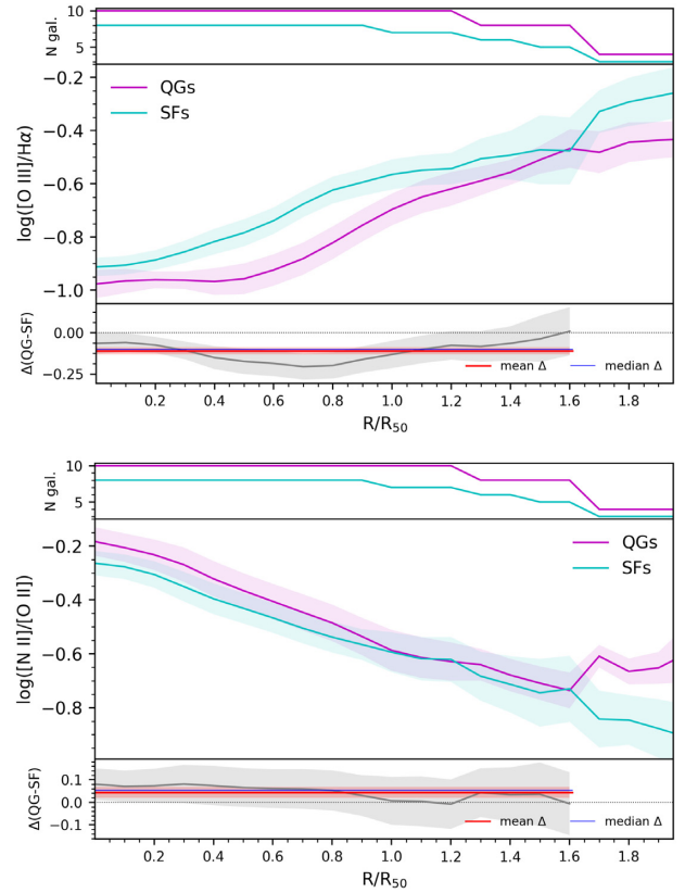
Figure 12. The average radial profiles of dust-corrected [O III]/H\alpha (top) and [N II]/[O II] (bottom) for QG and SF samples. The layout of the figure is the same as in Fig. 10.
