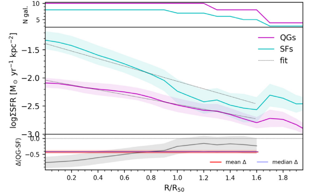
Figure 15. The SFR surface density ( \log \Sigma SFR) radial profile for QG and SF samples. The dotted black lines represent the linear fit to the radial profiles. The layout of the figure is the same as in Fig. 10.
