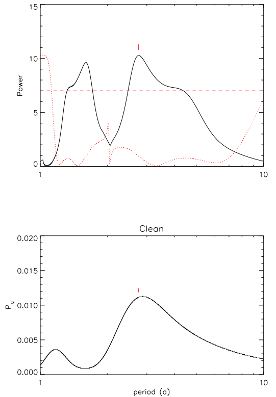
Fig. 4. Top panel: Generalized Lomb-Scargle periodogram of the g-band photometric time series of BD+20 1790. The solid black line is the normalized power versus period, the dotted red line is the spectral window, and the horizontal dashed line indicates the power level corresponding to a FAP = 0.01. Bottom panel: CLEAN periodogram. The red mark is the most powerful and significant peak in the periodogram.
