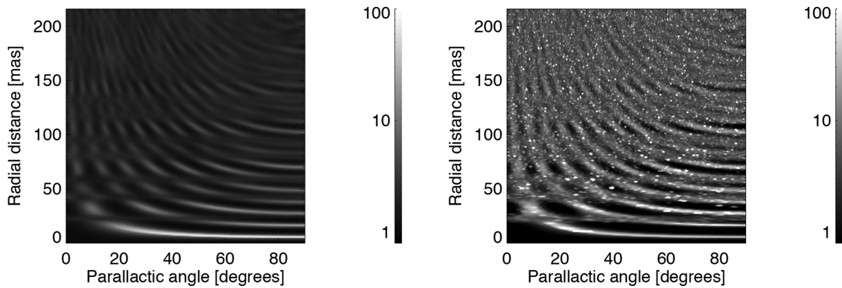
Figure 9. Contrast gain maps of the dual versus single aperture depending on the radial distance and the parallactic angle over 90^\circ . Long exposures ratio G_{LE} (left) and averaged short exposures ratio G_{SE} (right).
