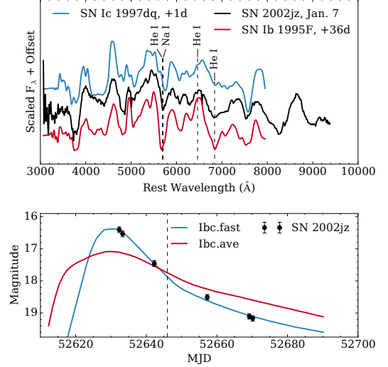
Figure 11. Top: spectrum of SN 2002jz from 2003-01-07 (corrected for a MW reddening of E(B - V) = 0.4846 \text{ mag} ) compared with that of SN Ic 1997dq and SN Ib 1995F (Matheson et al. 2001; Modjaz et al. 2014). Bottom: light curve of SN 2002jz compared to the stripped-envelope templates of L11, with the date of the spectrum shown with a vertical line.
