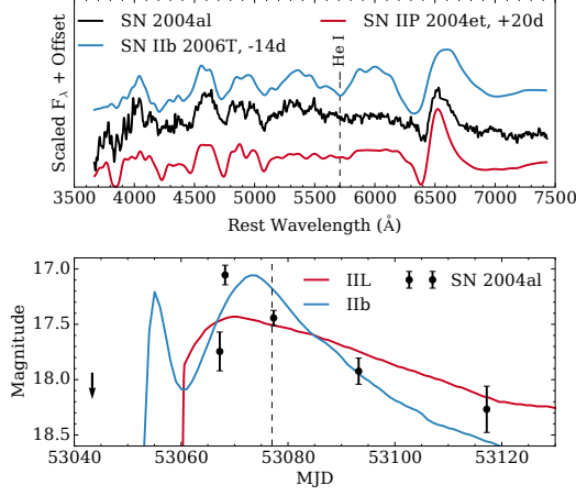
Figure 6. Top: spectrum of SN 2004al smoothed with a 20 Å Gaussian kernel and compared to spectra of the Type IIP SN 2004et a few weeks after maximum (Sahu et al. 2006) and the premaximum SN I Ib 2006T (the top non-IIP SNID template, Modjaz et al. 2014). Bottom: the light curve compared to templates from L11 with the date of the spectrum marked by a vertical line.
