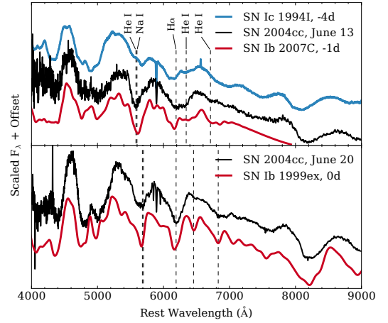
Figure 15. Top: spectrum of SN 2004cc observed on UT 2004-06-13 alongside premaximum spectra of SN Ic 1994I and SN Ib 2007C (Filippenko et al. 1995; Modjaz et al. 2014), and we mark He I lines at a velocity of 15,000 \text{ km s}^{-1} . Bottom: spectrum of SN 2004cc observed on UT 2004-06-20 and a spectrum of the Type Ib SN 1999ex (Hamuy et al. 2002), with the helium line marked at 10,000 \text{ km s}^{-1} , a deceleration consistent with the normal evolution of helium-line velocities in SNe Ib (Liu et al. 2016). Both spectra of SN 2004cc have been dereddened by E(B - V) = 1.0 \text{ mag} .
