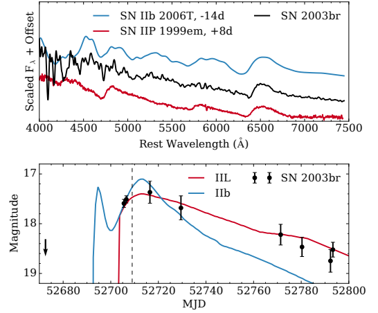
Figure 12. Top: spectrum of SN 2003br (corrected for E(B - V) = 1.0 \text{ mag} and smoothed with a 40 \text{ \AA} Gaussian kernel), compared to that of the Type I Ib SN 2006T (Modjaz et al. 2014) and the Type IIP SN 1999em (Leonard et al. 2002b) — both match well. Bottom: the light curve compared to the templates from L11, with the date of the spectrum marked.
