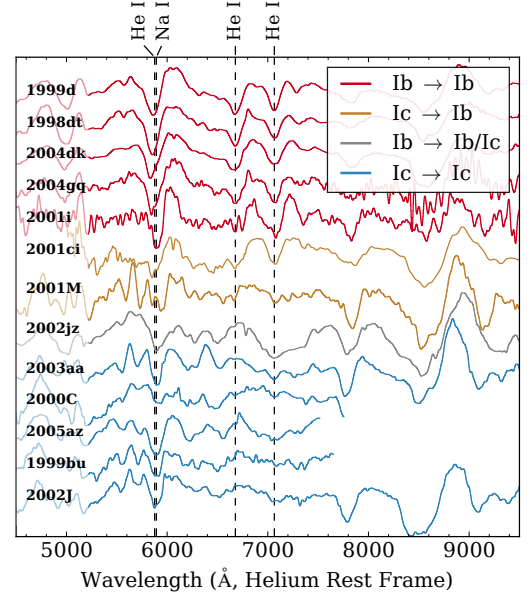
Figure 1. Representative sample of spectra of the SNe Ib and Ic in our sample, observed between 5 and 20 days after peak brightness, as well as spectra of three SNe for which we provide updated classifications (SNe 2001M, 2001ci, and 2002jz). We have subtracted a spline continuum from these spectra, smoothed them with a 50 Å Gaussian kernel, and shifted them in velocity space to align their He I features (or Na I \lambda 5892 if no helium is detected).
