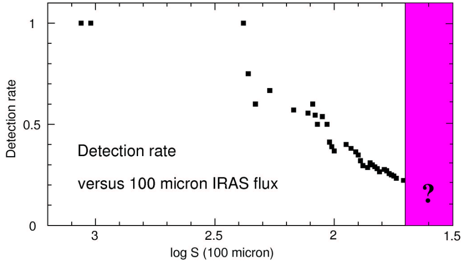
Fig. 1. Detection rate of the H 2 O FIR-maser sample including all galaxies above a given 100 μm IRAS Point Source Catalog flux density (Peck et al. 2004).
