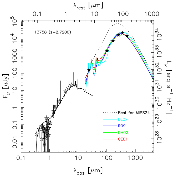
Figure 21. Example of a UV-to-FIR SED. The black line shows the best-fit BC03 stellar population model for the photometry up to 8\ \mu\text{m} rest frame (open black stars), which provide an estimate of the stellar population properties and the dust attenuation. The filled black stars show the mid-to-far-IR data from Spitzer MIPS and Herschel PACS and SPIRE. The red, green, blue, and cyan lines show the best-fit dust emission models from the libraries of Chary & Elbaz (2001), Dale & Helou (2002), Rieke et al. (2009), and Draine & Li (2007), which provide similar results. The dashed line shows the fit to only the MIPS 24\ \mu\text{m} data. The significant difference between this and the other templates illustrates why using an average-luminosity template, as in the Wuyts et al. (2011b) method, is a better approach for MIPS-only SEDs.
