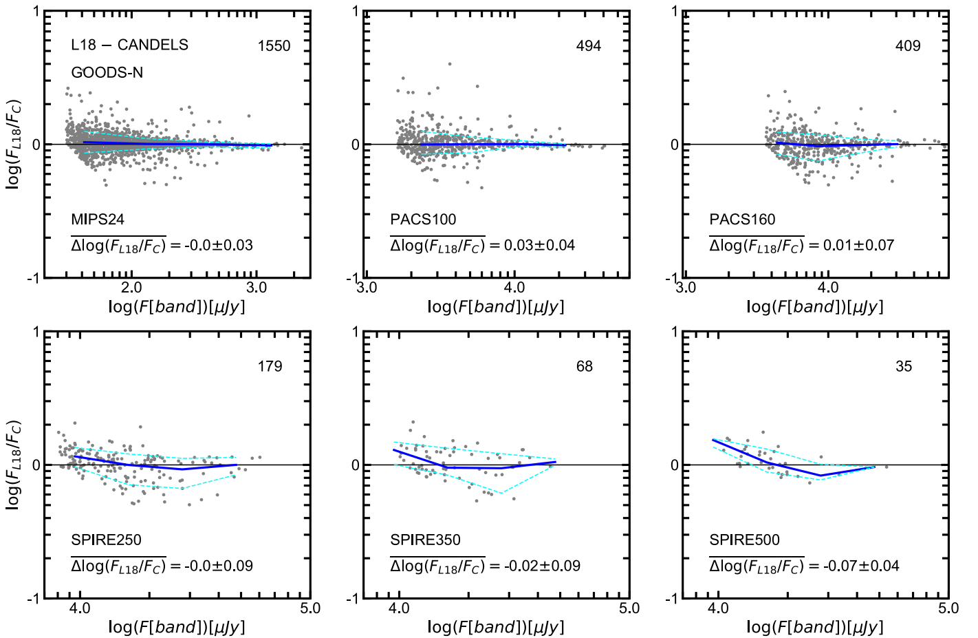
Figure 29. Comparison of mid-to-far-IR fluxes between the CANDELS (this work) and the Liu et al. (2018) catalogs in the GOODS-N field. From left to right and top to bottom, the panels show the comparison of the MIPS24, PACS100, PACS160, SPIRE250, SPIRE350, and SPIRE500 fluxes. The y axis shows the differences in L18 minus CANDELS values. The comparison is restricted to galaxies detected above S/N = 5 in each band in both catalogs (see Table 13). The blue lines show the running median and \pm 1\sigma scatter of the distribution whose average values are indicated in the bottom-left corner. The values in each panel have been corrected by a constant offset derived from the average running median. The declining sensitivity and spatial resolution with increasing wavelength of the bands lead to fewer detections, larger scatter, and some outliers likely caused by differences in the deblending of particularly crowded sources. Nonetheless, we find an overall good agreement in all bands with systematic offsets smaller than \sim 0.1 dex and a scatter that is roughly consistent with photometric uncertainties.
