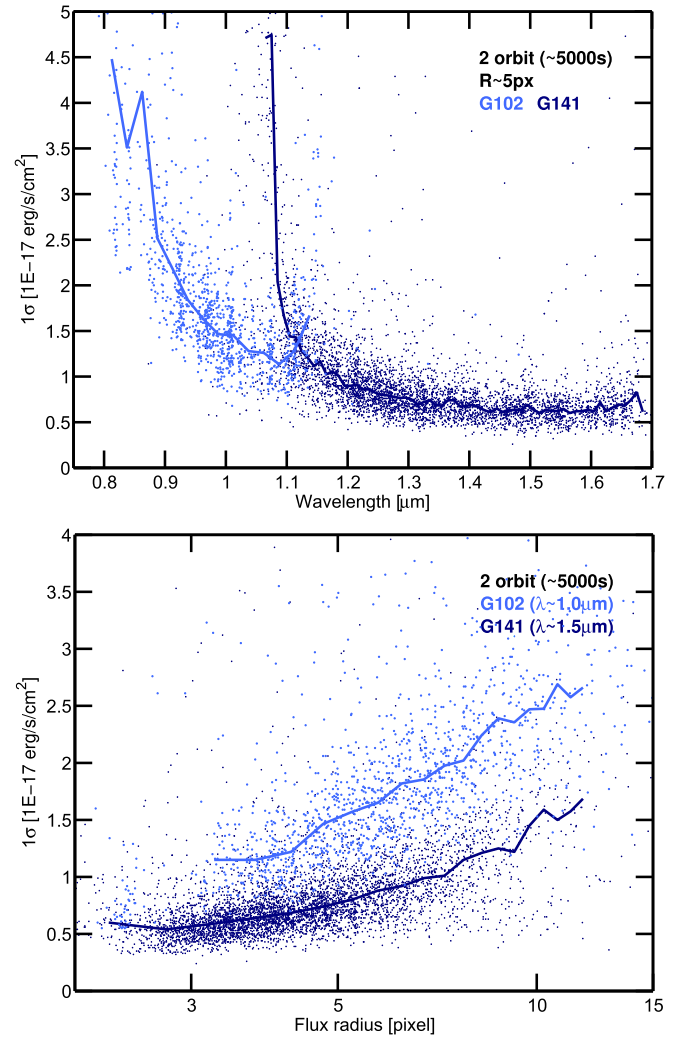
Figure 14. 1\sigma emission-line sensitivity in the G102 and G141 spectra as a function of the observed wavelength (upper panel) and the SExtractor flux_radius size of the galaxies (lower panel). In order to illustrate the effect of the two main drivers of emission-line sensitivity separately, the upper panel shows galaxies with similar sizes of R \sim 5 pixels, typical for resolved galaxies, while the bottom panel shows galaxies with emission lines measured around the same wavelengths, \lambda \sim 1.0 and 1.5 \mu\text{m} for G102 and G141. At those wavelengths, the average line uncertainty of the two-orbit-depth grism spectra for a resolved galaxy are 0.75 and 1.5 \times 10^{-17} \text{ erg s}^{-1} \text{ cm}^{-2} in G141 and G102, respectively.
