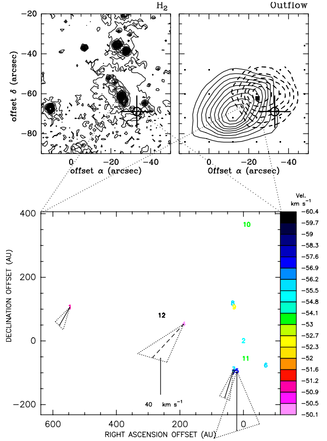
Fig. 2. WB89-234. ( Upper panels ) TIRGO H 2 2.12 \mu m image (left); blue (dashed lines) and red (solid lines) lobes of 12 CO(1–0) wing emission (right); the big cross and the filled square indicate respectively the Effelsberg and VLA positional uncertainties of the H 2 O maser. ( Bottom panel ) VLBI 22 GHz water maser features (see the caption of Fig. 1).
