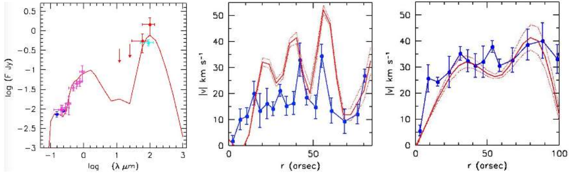
Fig. 7. Left: measured (filled dots) and predicted (red solid line) SED of the NGC 3447A/NGC 3447 system; blue, magenta, red, and azure dots indicate far-UV GALEX, from Marino et al. (2010), Swift-UVOT and SDSS (Tables 1 and 2), IRAS and AKARI-F (Catalog Archive Server, Yamauchi et al. 2011) data, respectively. Middle and right: comparison between the observed velocity profiles along the directions in Fig. 4, PA = 14.3° ( middle ) and PA = 65° ( right ), with those derived from the selected snapshot in the corresponding directions and within the same semi-angle sector (i.e. 25°). The velocity profiles are folded and rebinned within 5'' (blue filled dots) to be compared with the same slices of the simulation (red solid and dotted lines), with the same binning.
