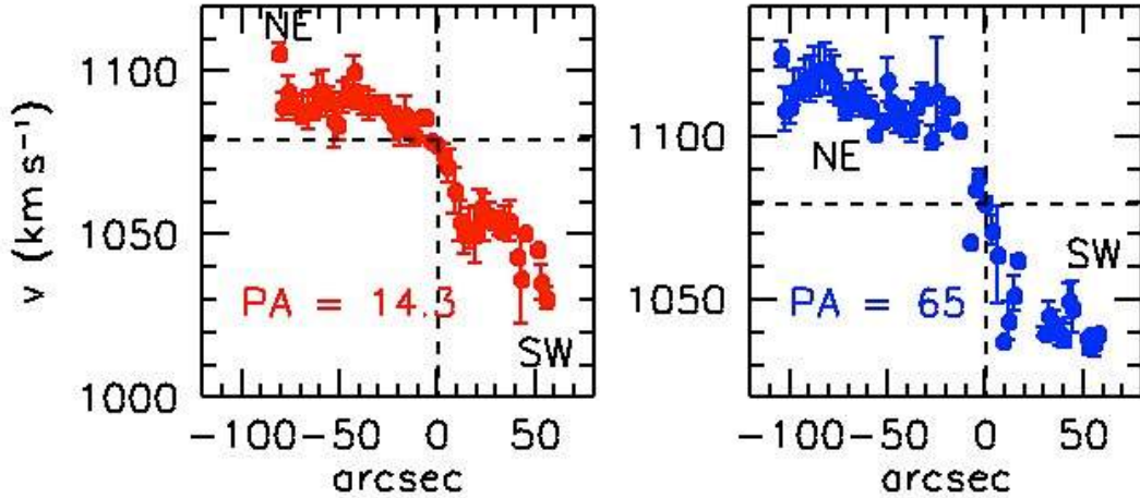
Fig. 4. Velocity profiles along the lines of sight in Fig. 3 (top left panel) corresponding to PA = 14.3^\circ , and PA = 65^\circ which connects NGC 3447A; horizontal dashed lines indicate the derived systemic velocity ( 1079 \text{ km s}^{-1} , Sect. 2.3).
