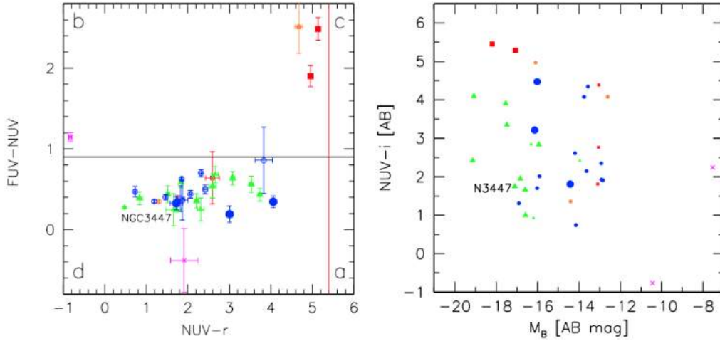
Fig. A.2. Colour-colour diagram, \text{NUV} - r vs. \text{FUV} - \text{NUV} (left panel) and the colour-magnitude diagram, M_B vs. \text{NUV} - i (right panel), for all the LGG 225 members; (red) squares indicate ETGs ( T \leq -2 ), (orange) diamonds S0s ( -2 > T \geq 0 ), (green) triangles Spirals ( T < 9 ), (blue) circles show Irregulars ( T \geq 9 ) and magenta crosses are for galaxies without morphological classification in the Hyperleda catalogue; small dots are for new members of this work (Table A.2). Solid lines (left) correspond to the conditions \text{FUV} - \text{NUV} < 0.9 , that is, UV rising slope, and \text{NUV} - r > 5.4 shows the region of young massive star-free galaxies. These conditions, following the UV classification scheme by Yi et al. (2011), separate passive evolving ETGs (region c) from star forming galaxies (region a), see text. In both panels magnitudes were corrected by galactic extinction following Burstein & Heiles (1982).
