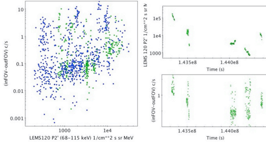
Fig. 12 Same as Figure 11 but for the EPIC MOS2 and ACE LEMS120 P2' data taken in time intervals affected by SEP events when XMM was outside of the bow shock. Highlighted in green and shown in the light curves are the data taken during the SEP period of 16-30 July 2002 for 165 ks.
