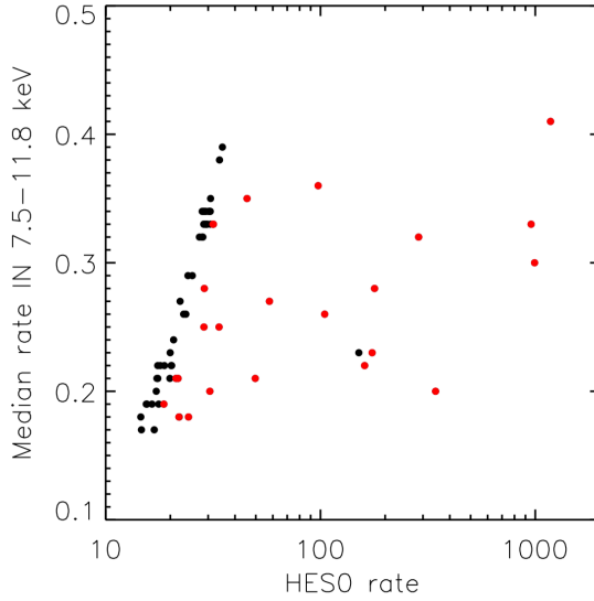
Fig. 4 Correlation of the ERM HES0 count rate and the corresponding median rate over the all inFOV for closed observations. The black points show the expected correlation when the HES0 count rate is representative of the GCR flux. Red points are selected when filtering for SEPs or radiation belts passage as detailed in the following section.
